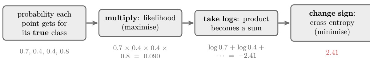
Figure 3: From probabilities to cross entropy
