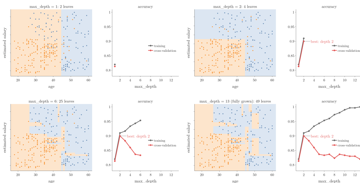
Figure 3: max_depth from 1 to 13 (fully grown) on the Social Network Ads data. Left: the decision surface. Right: training accuracy and 5-fold cross-validation accuracy on the 300 training observations
