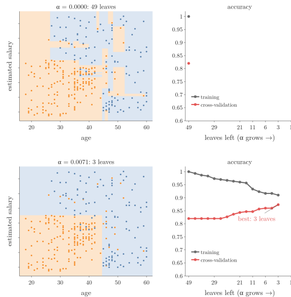
Figure 7: Cost-complexity pruning of the fully grown Social Network Ads tree, one value of \alpha per frame. Left: the decision surface. Right: training accuracy and 5-fold cross-validation accuracy against the number of leaves left. Cross-validation picks the 3-leaf tree.
