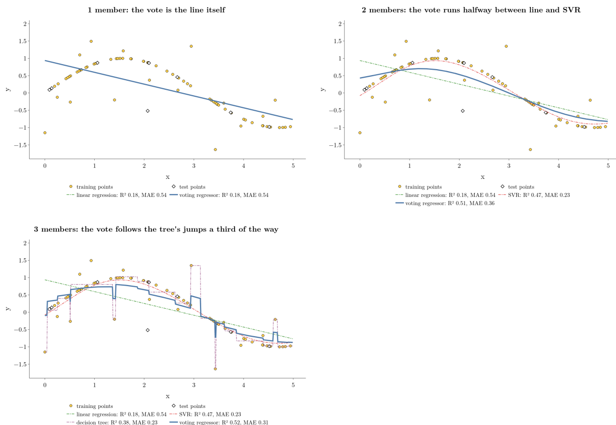
Figure 2: Base regressors (dash-dot) added one at a time on the noisy sine data, and the voting regressor (solid blue) after each addition: the line alone, then halfway between line and SVR, then the mean of line, SVR and tree. Legends give R^2 and MAE on the 8 test points
