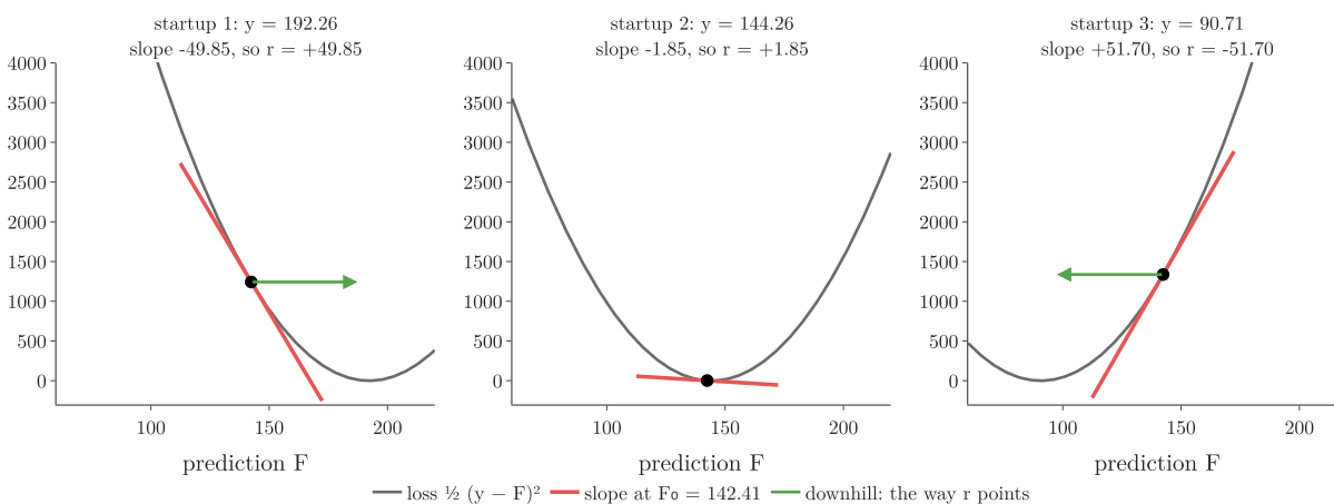
Figure 5: Each startup’s loss \frac{1}{2}(y - F)^2 against the prediction F . The red line is the slope at F_0 = 142.41 ; the pseudo-residual is minus that slope, and the green arrow is the downhill direction
