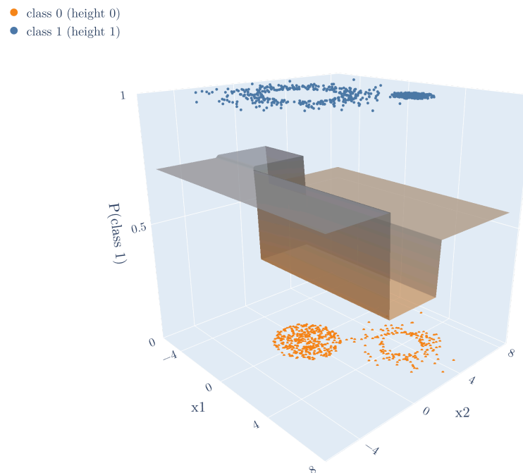
Figure 10: The data lifted to height 0 (class 0) or 1 (class 1), with the model's probability surface after one tree
