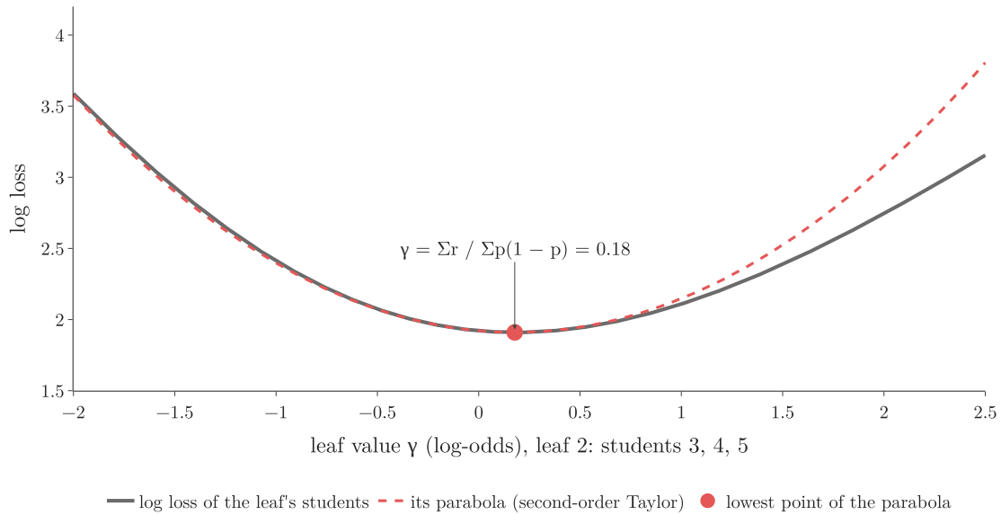
Figure 6: The log loss of leaf 2's students against the leaf value \gamma (grey), its second-order Taylor parabola (dashed red), and the parabola's lowest point: the leaf value 0.18
