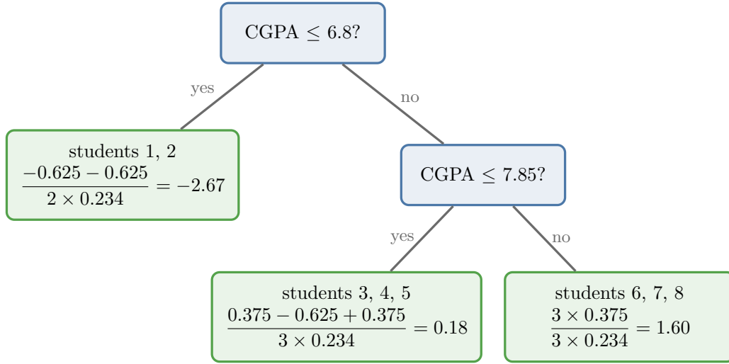
Figure 5: Tree 1 with the log-odds value of each leaf
