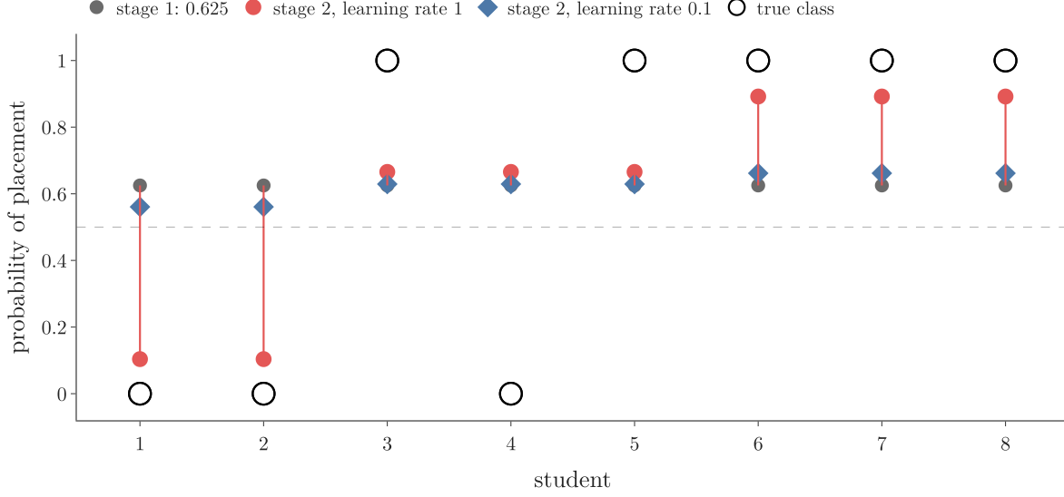
Figure 7: Probability of placement after stage 2, learning rate 1 (red dots, with the move from stage 1 as a red line) and 0.1 (blue diamonds); open circles mark each student’s true class
