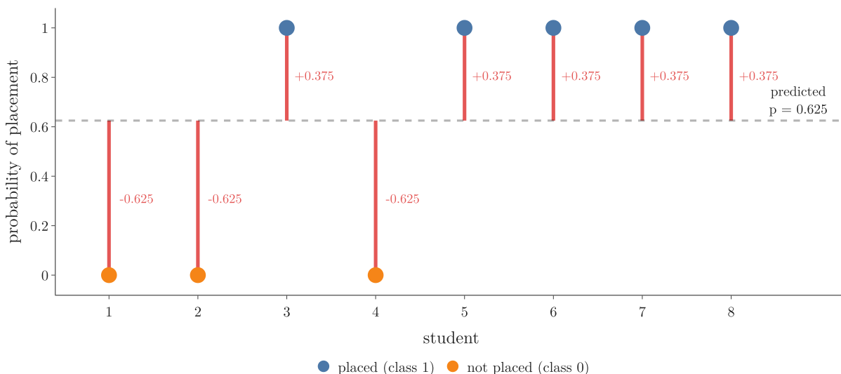
Figure 3: The eight students at stage 1: true class (dots), predicted probability 0.625 (dashed line) and the pseudo-residuals y - p (red gaps). Drawing residuals as gaps to a probability line follows StatQuest, “Gradient Boost Part 3 (of 4): Classification”
