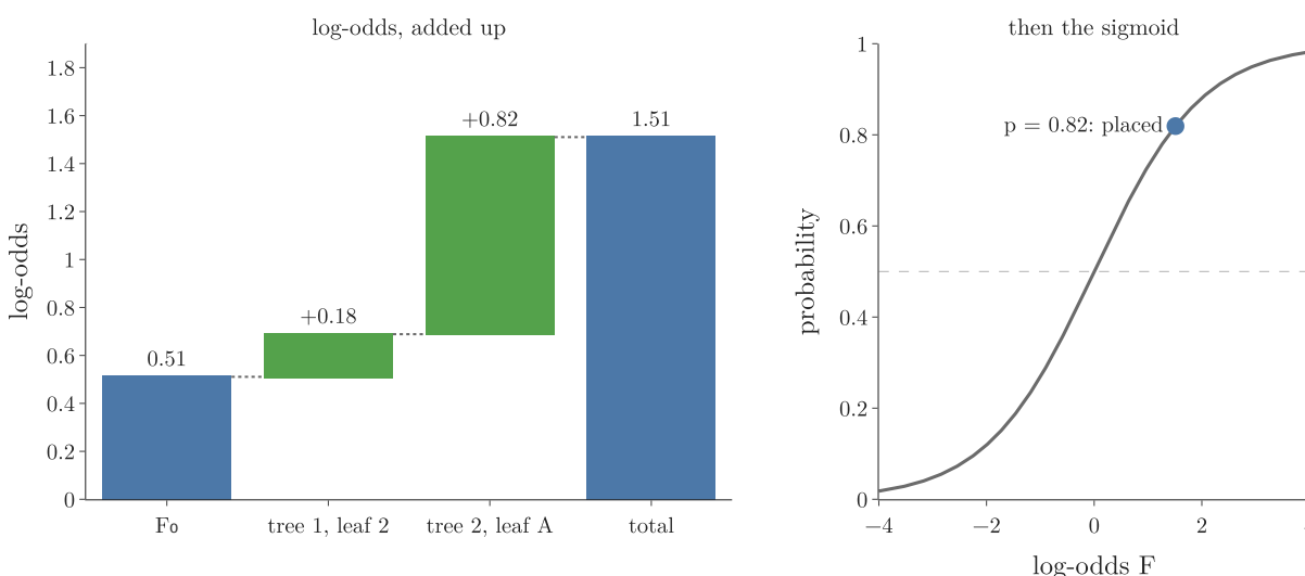
Figure 9: The new student (CGPA 7.2, IQ 100): F_0 = 0.51 plus 0.18 from tree 1 and 0.82 from tree 2 gives log-odds 1.51 (left); the sigmoid turns it into probability 0.82 (right)
