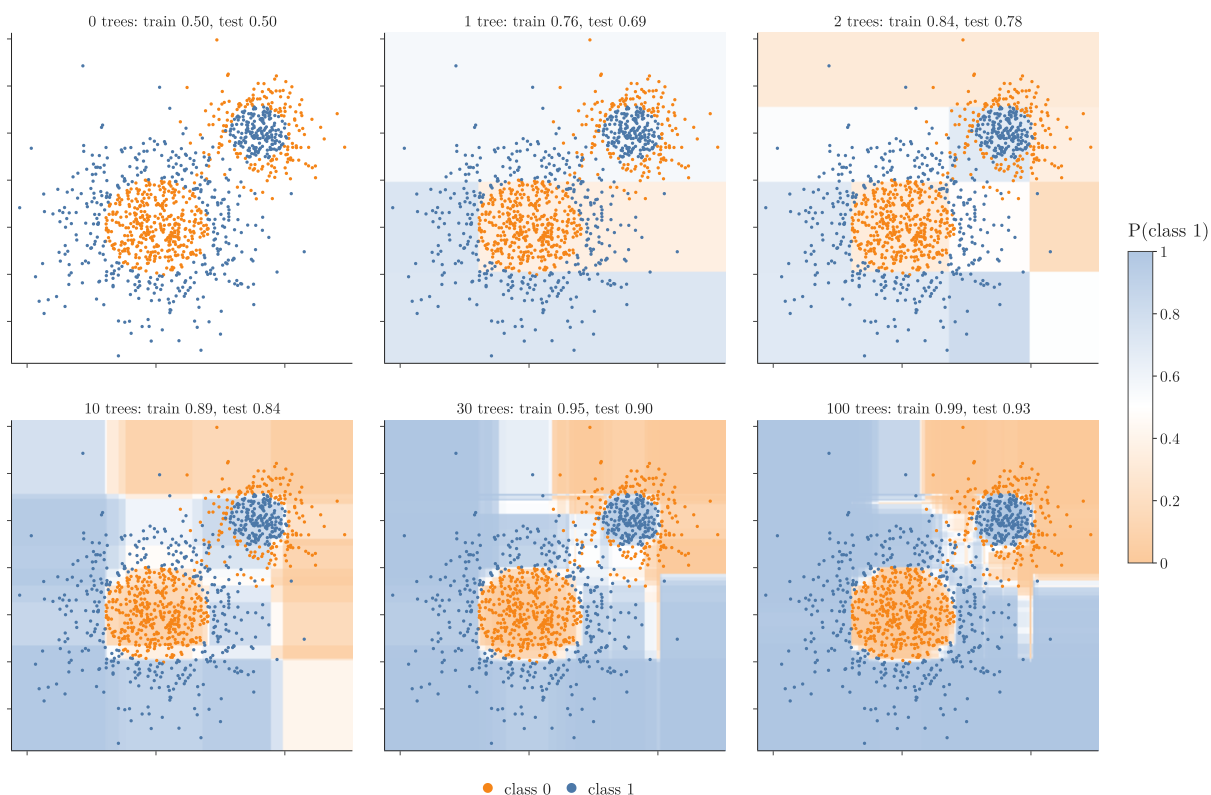
Figure 11: Probability of class 1 after 0, 1, 2, 10, 30 and 100 trees (learning rate 0.5, 4 leaves per tree); blue above 0.5, orange below
