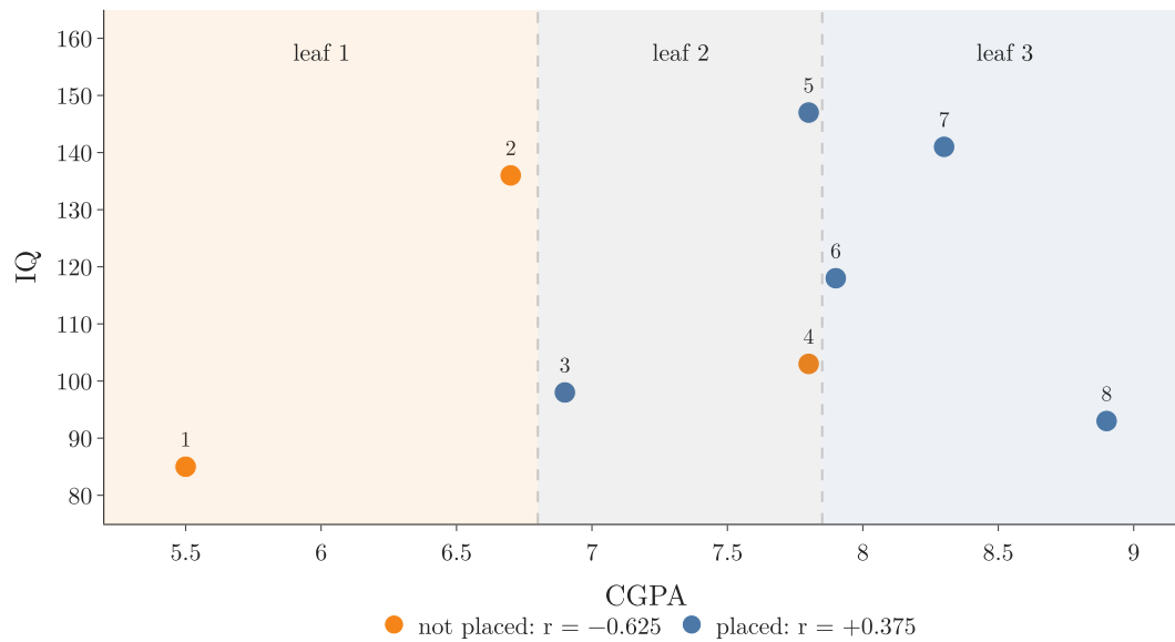
Figure 4: Tree 1’s three leaves as bands of CGPA over the eight students (numbered); orange students have residual -0.625 , blue ones +0.375
