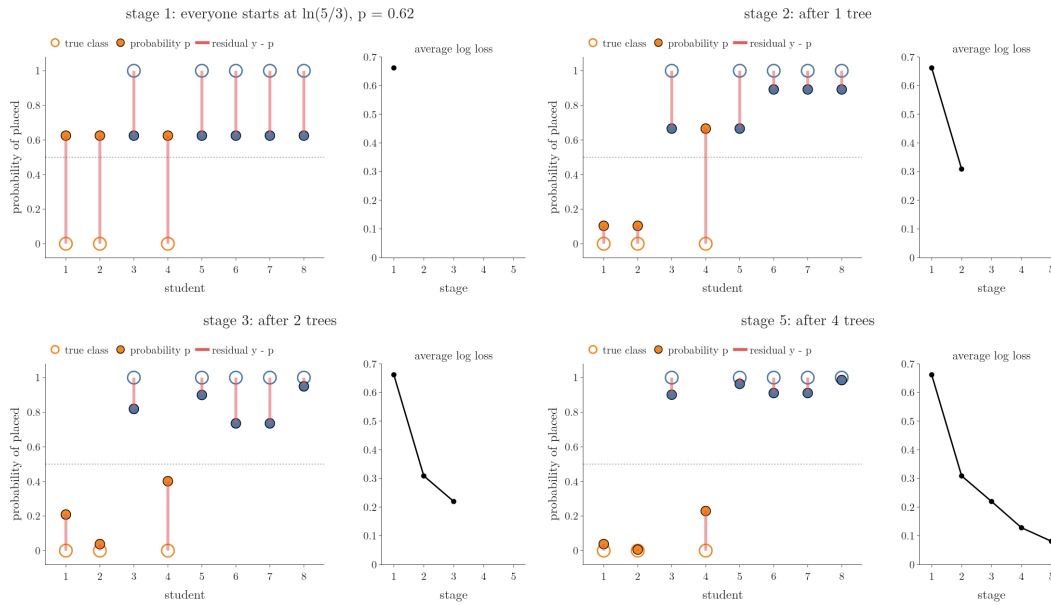
Figure 8: Each student's probability of placement (filled dot) moves towards its true class (ring) stage by stage; the red bar is the pseudo-residual y - p that the next tree learns. Right: average log loss. Learning rate 1, trees with 3 leaves, as in the tables. Drawing residuals as bars to the true class follows StatQuest's "Gradient Boost Part 3: Classification" (Starmer)
