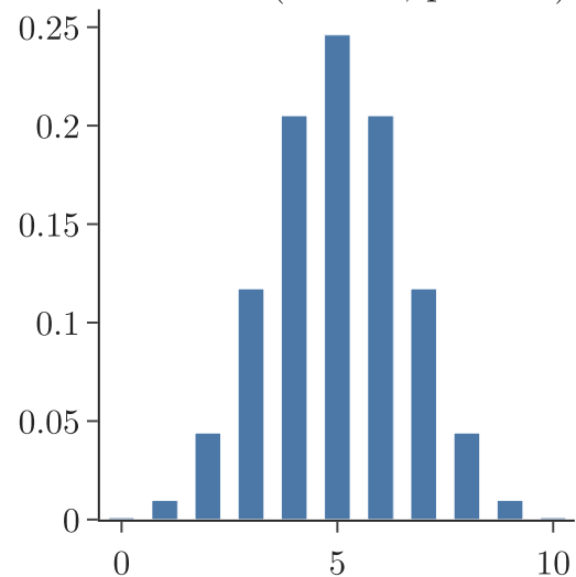
Binomial ( n = 10, p = 0.5 )
