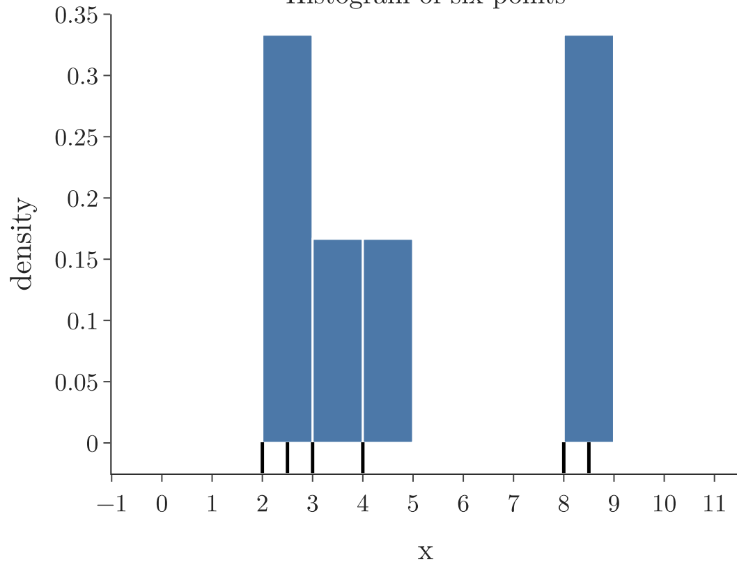
Histogram of six points
