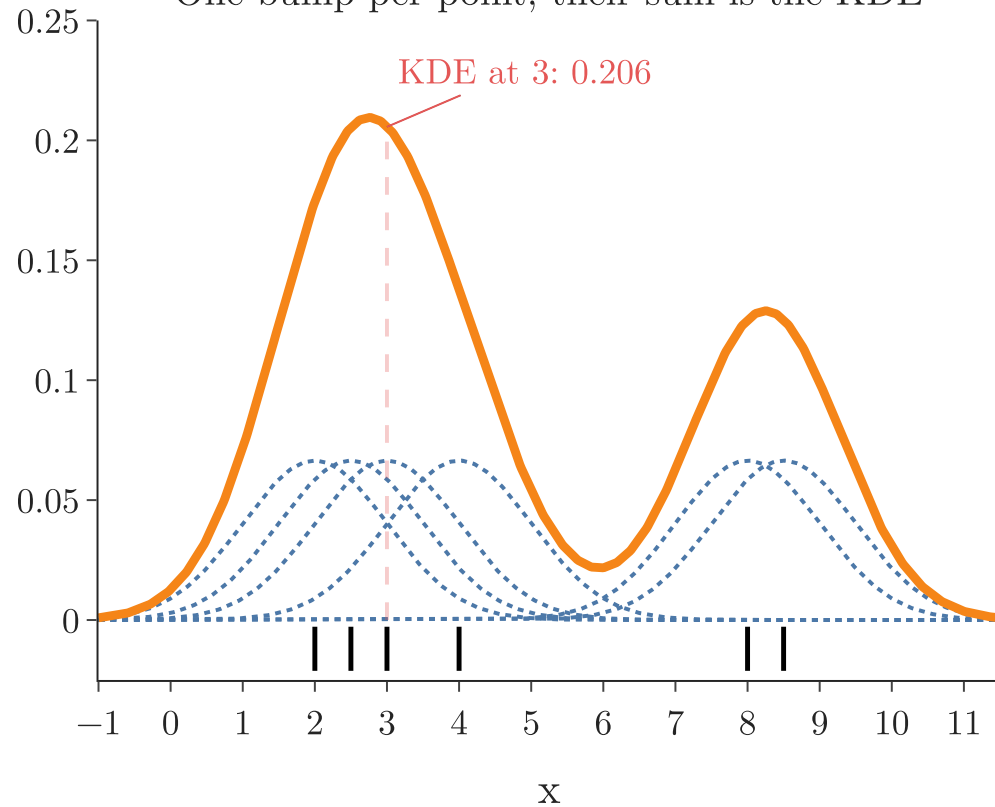
One bump per point; their sum is the KDE
