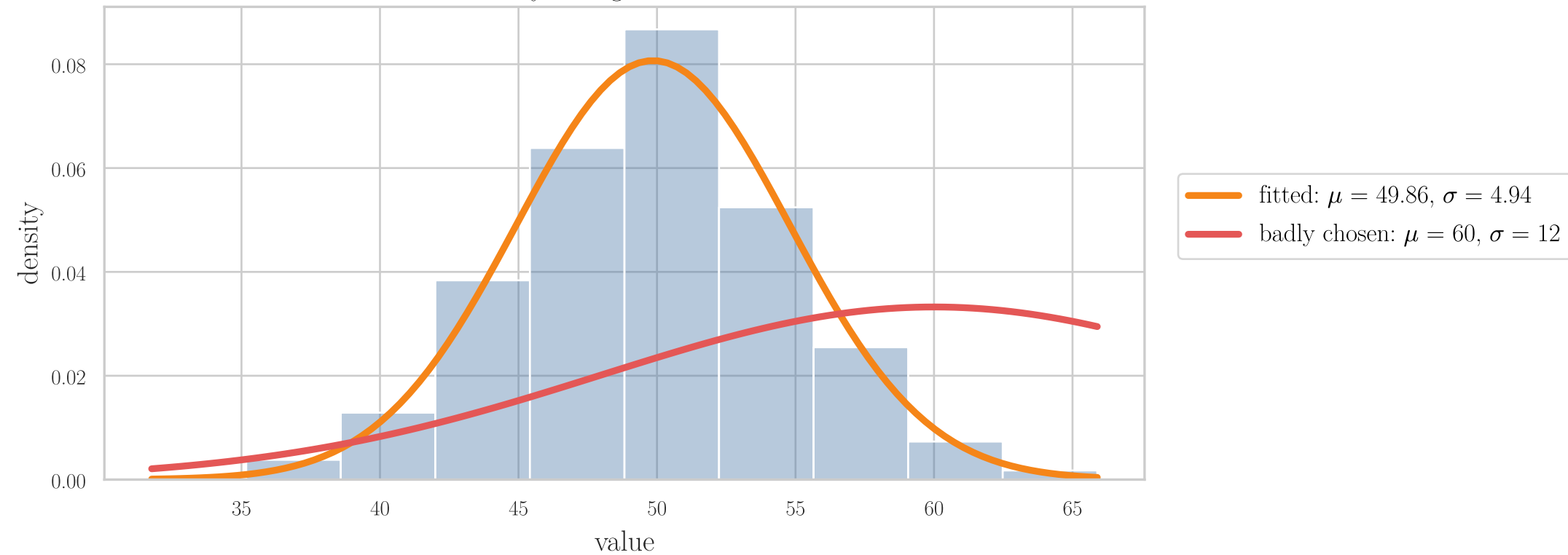
1000 values: density histogram and two normal PDFs
