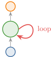
RNN / LSTM
