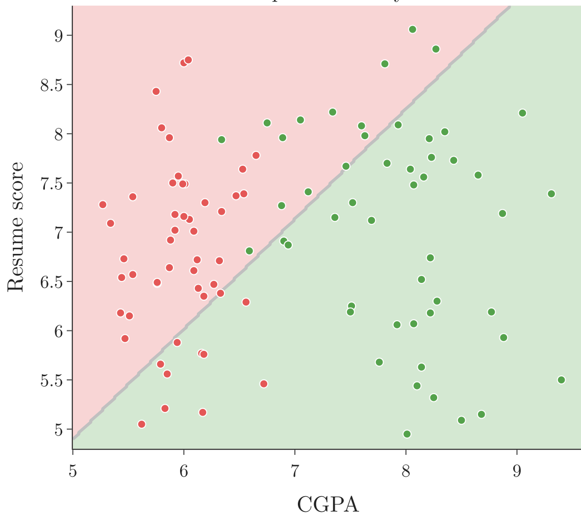
Raw inputs: accuracy 75%
