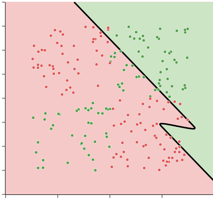
XOR: 2 hidden nodes, sigmoid accuracy 69%
