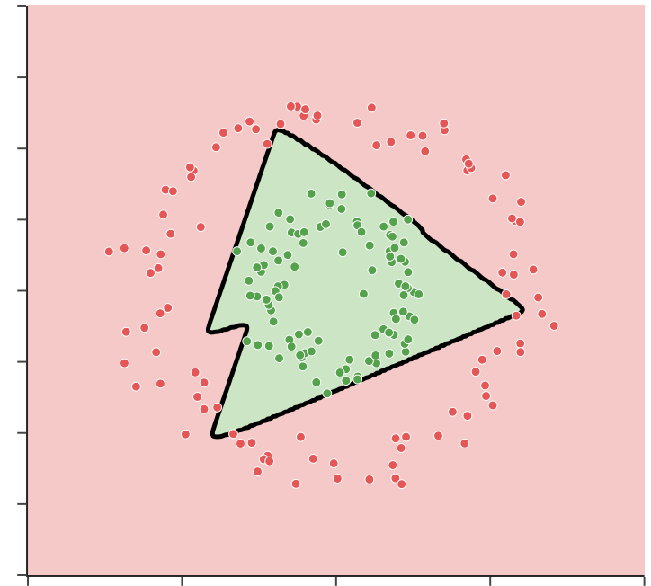
Circles: 4 hidden nodes, sigmoid accuracy 100%
