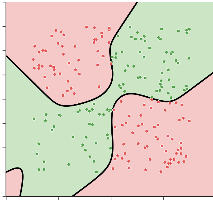
XOR: 4 hidden nodes, sigmoid accuracy 100%
