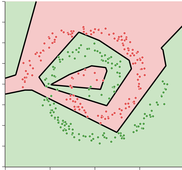
Spiral: 4 layers of 4, ReLU accuracy 99%
