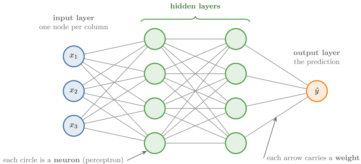
Figure 1: The parts of an artificial neural network: input layer, two hidden layers, output layer
