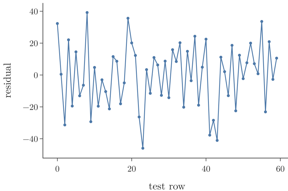
5. No autocorrelation: residuals in order
