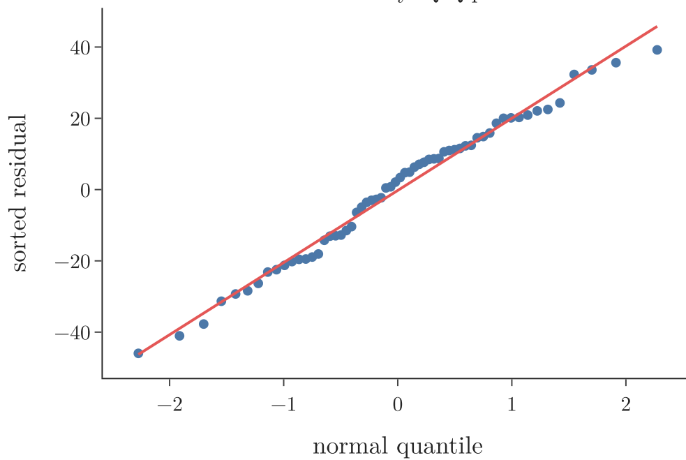
3. Normality: Q-Q plot
