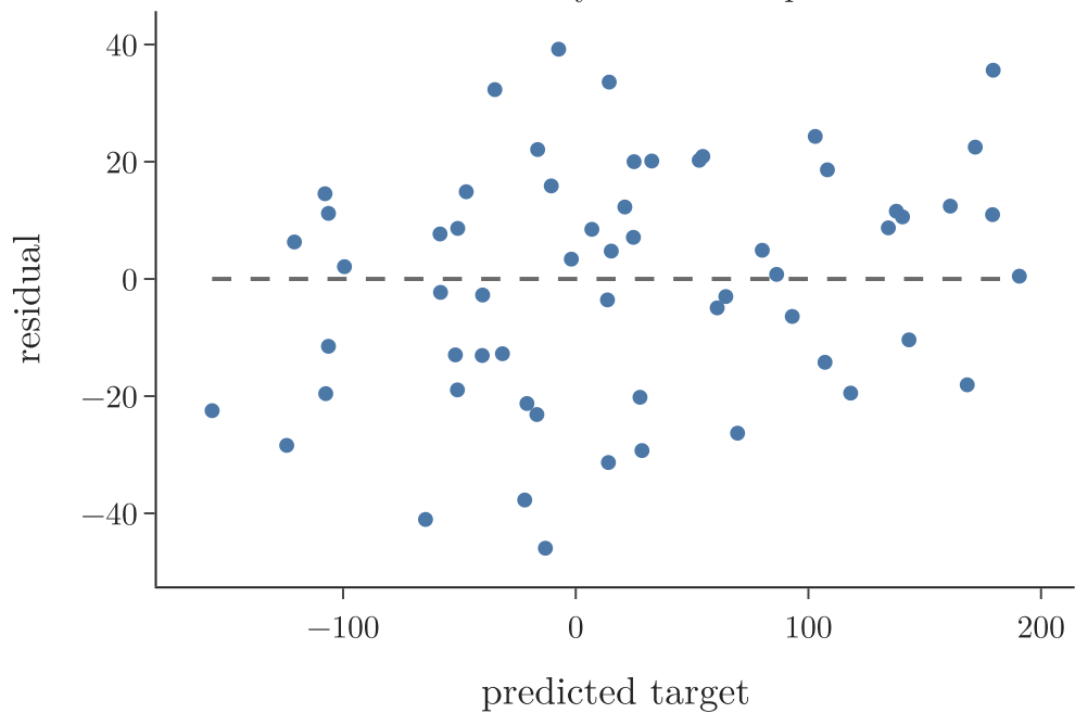
4. Homoscedasticity: residual vs prediction
