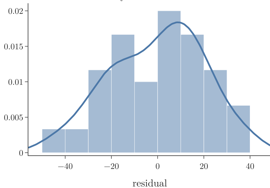
3. Normality: distribution of residuals
