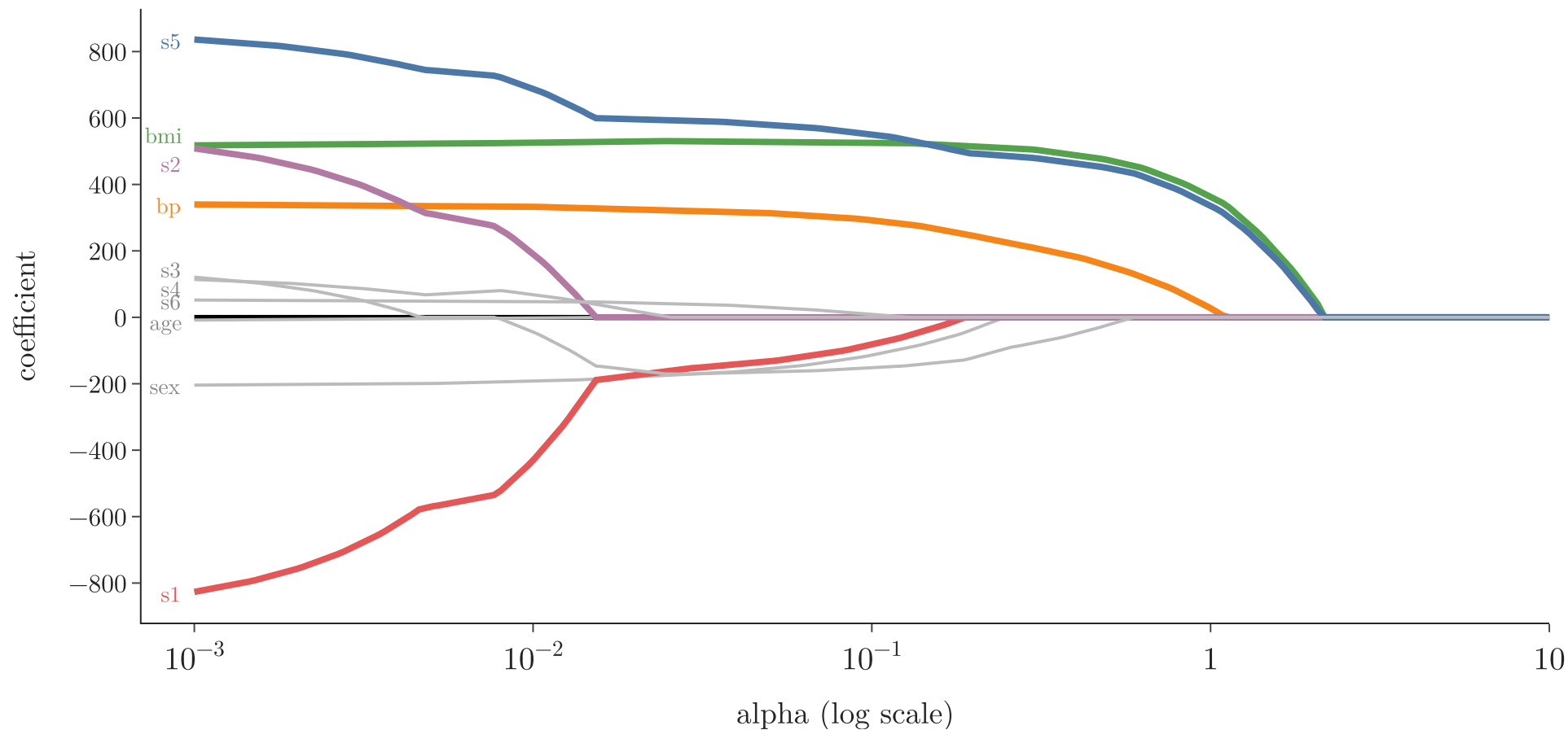
Lasso: coefficients hit 0 one by one; bmi and s5 survive longest
