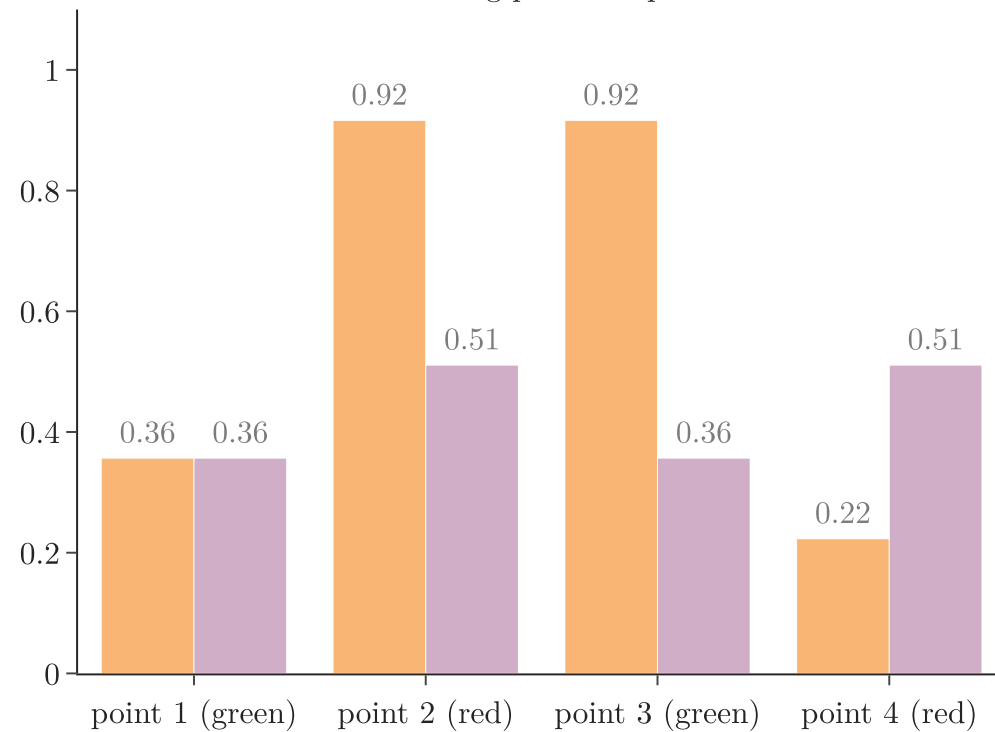
Cost -\log p of each point
