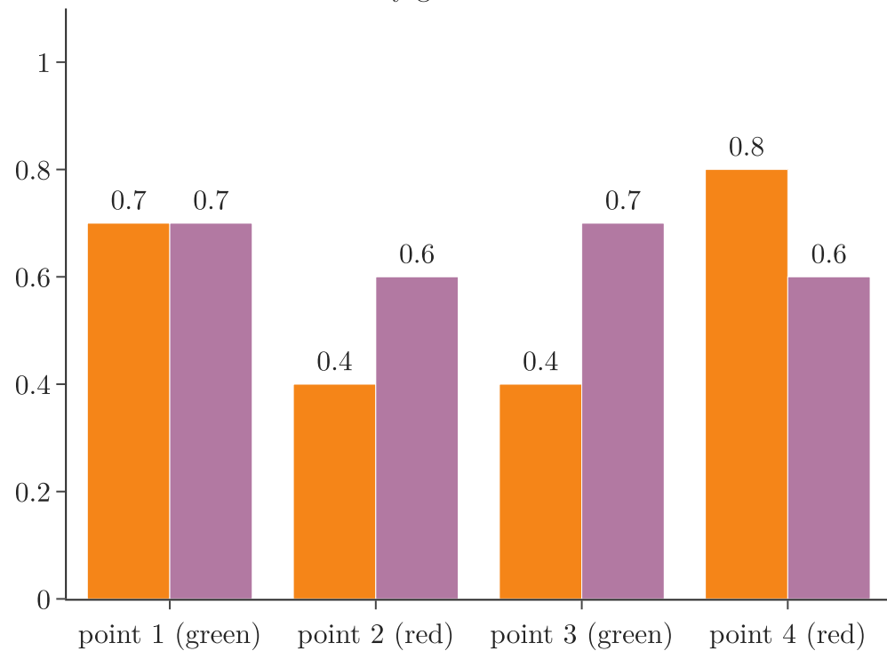
Probability given to the true class
