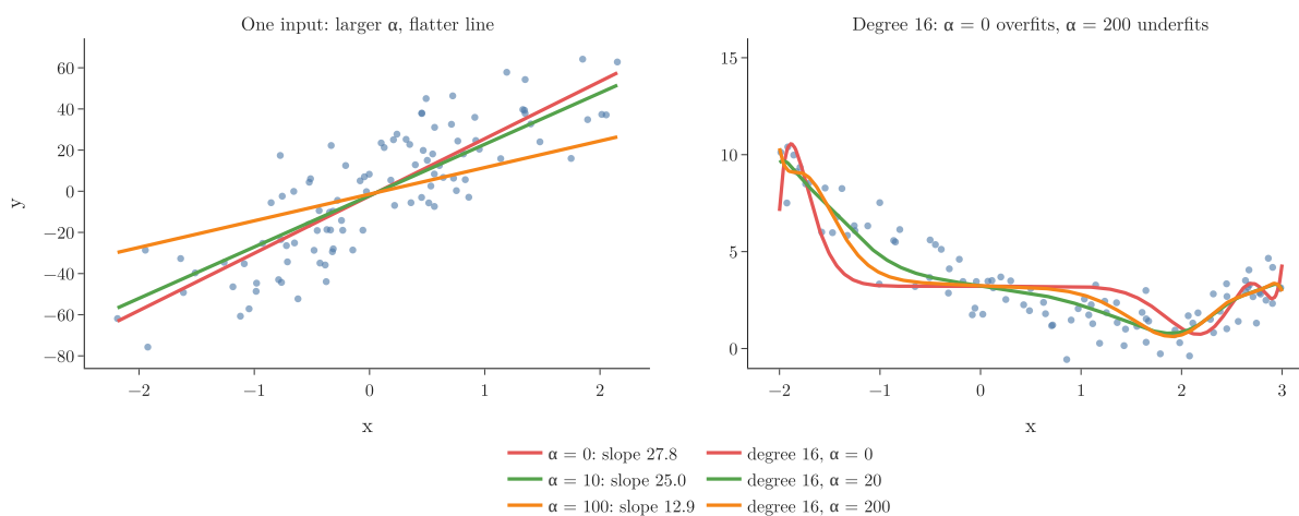
Figure 2: The effect of alpha with one input and with a degree-16 polynomial
