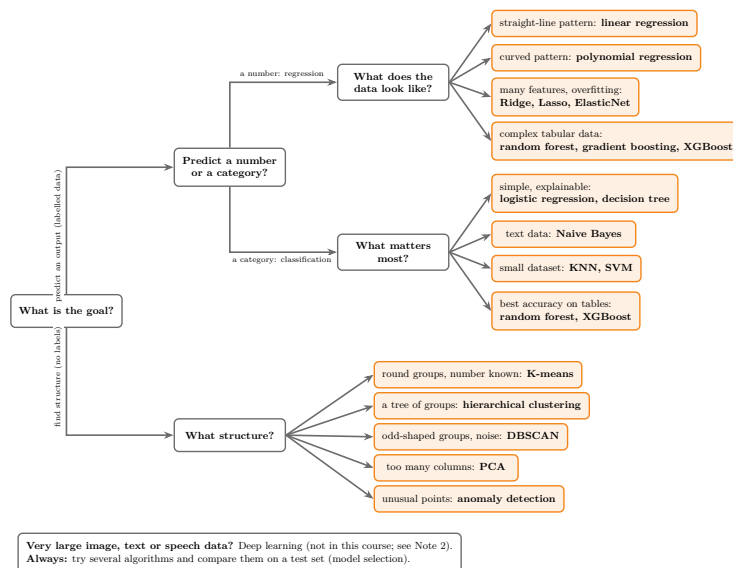
Figure 8: The Algorithm chooser (draft)
