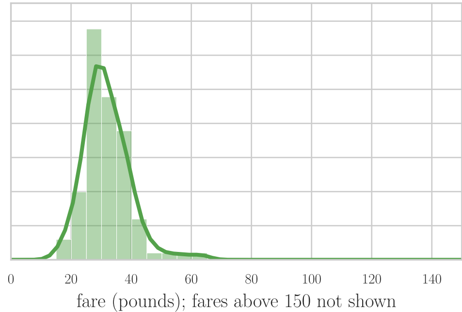
100 sample means, n = 50
