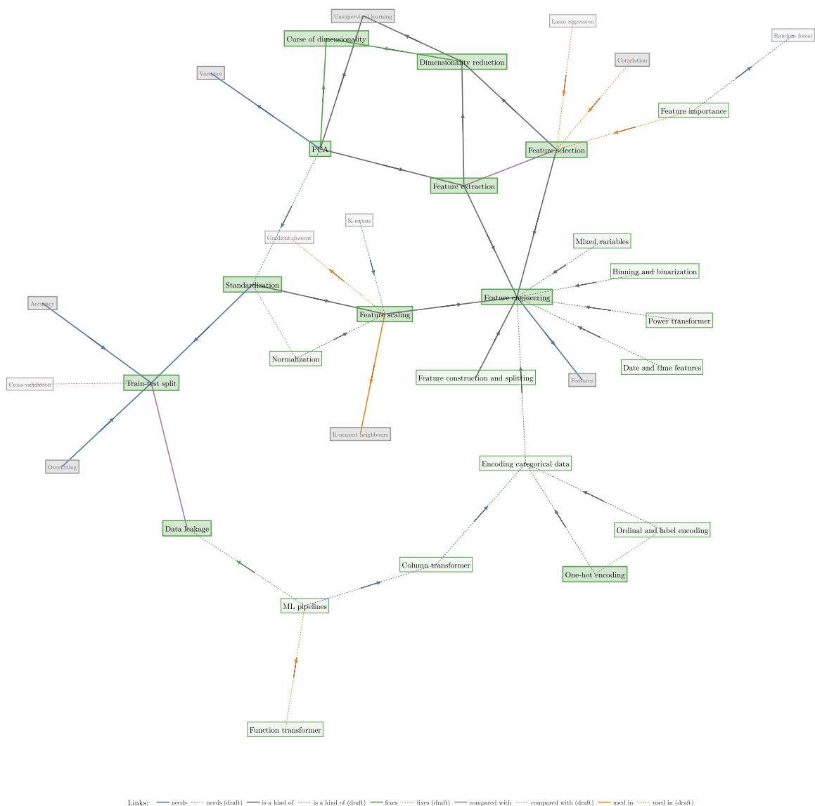
Figure 4: Concept map: Features, dimensions and splitting
