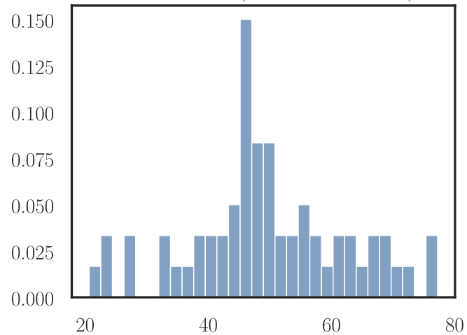
no pattern (too many bins)
