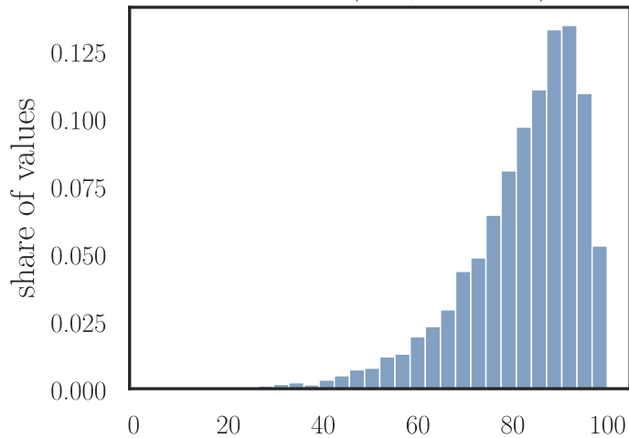
left skew (long tail left)
