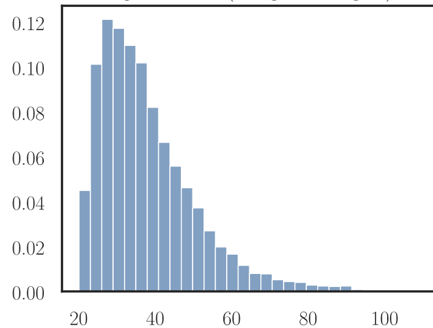
right skew (long tail right)
