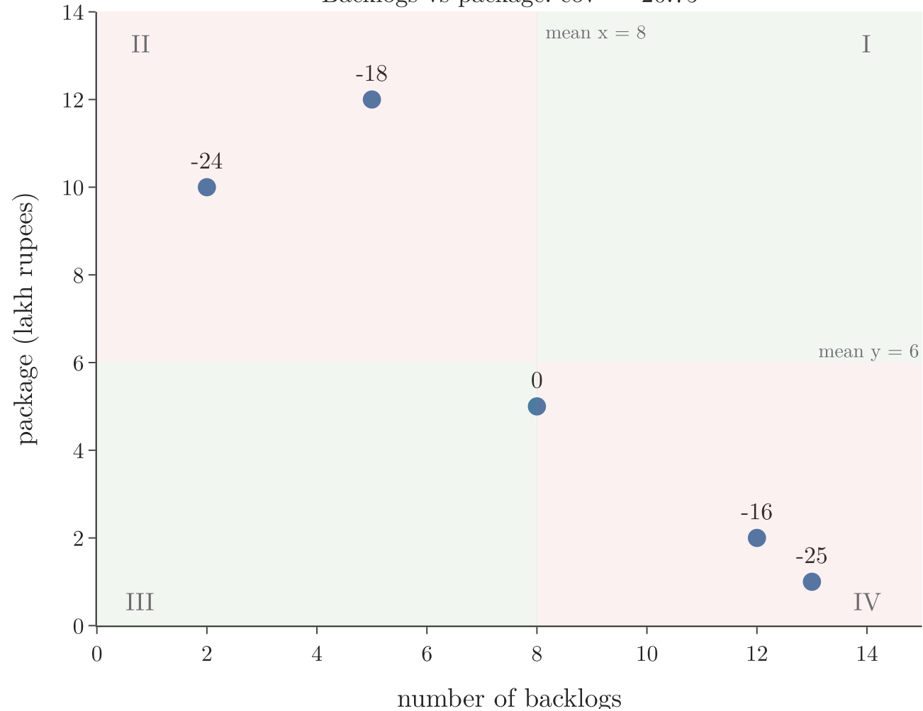
Backlogs vs package: cov = -20.75
