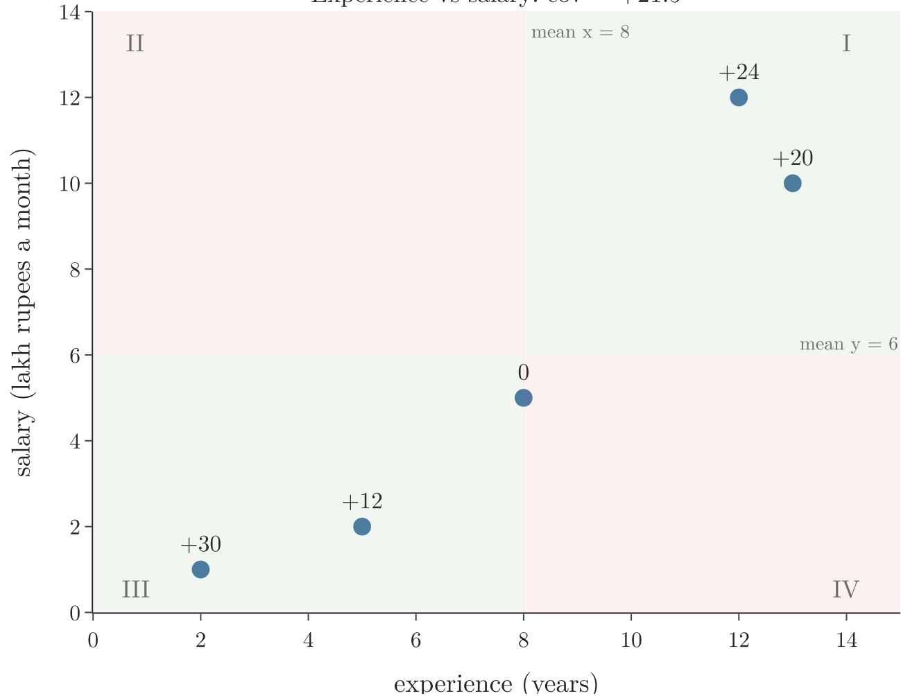
Experience vs salary: cov = +21.5
