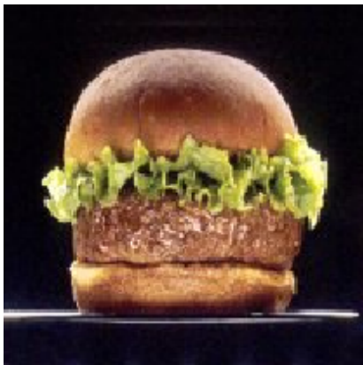
cheeseburger 1.00
