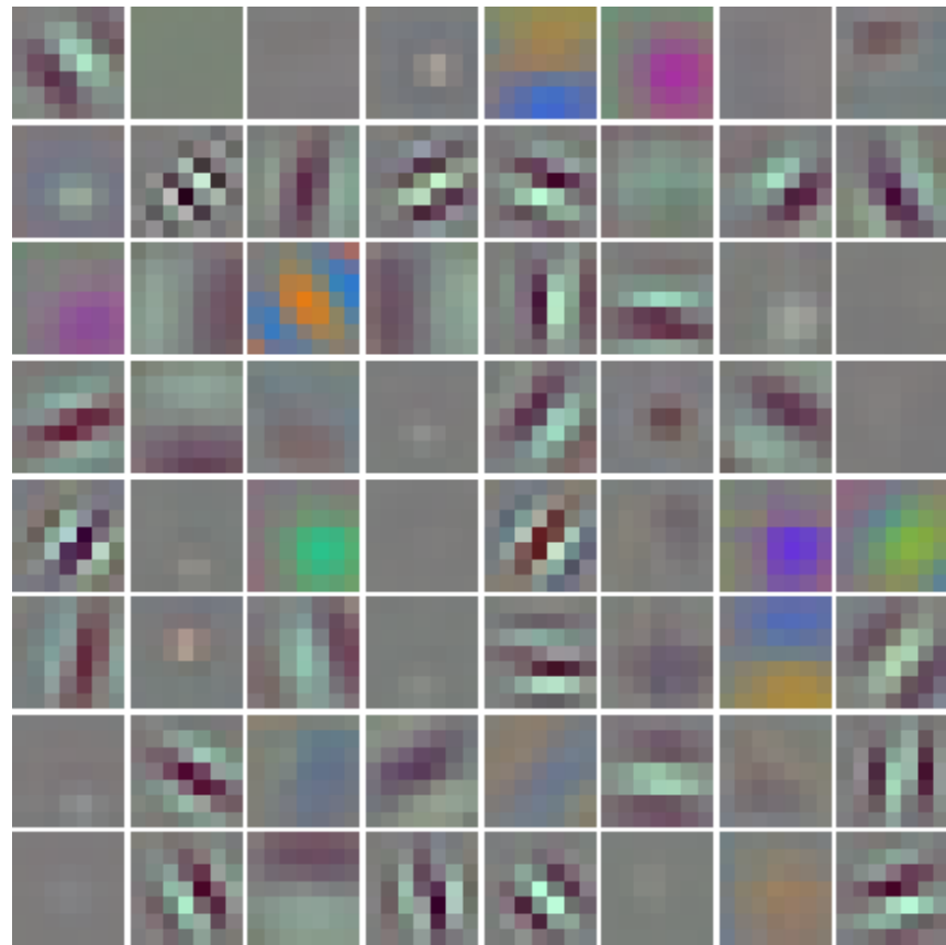
ResNet50, first layer: 64 filters of 7 x 7
