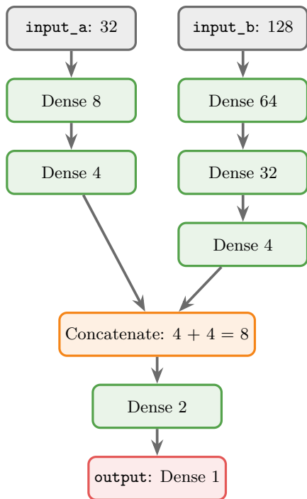
(a) Two inputs, one output
