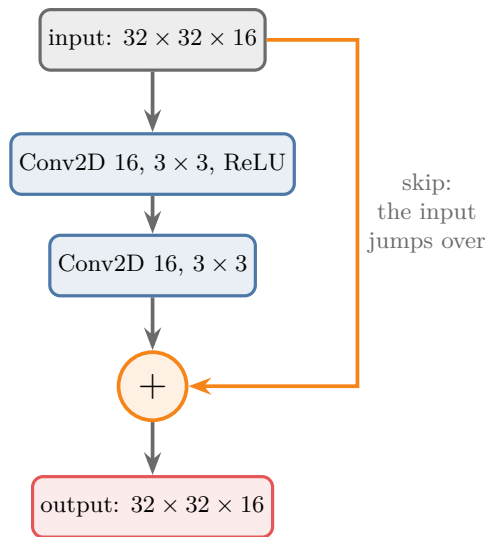
(b) A skip connection
