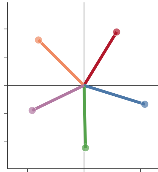
ReLU, S = 0.95 5 of 5 stored
