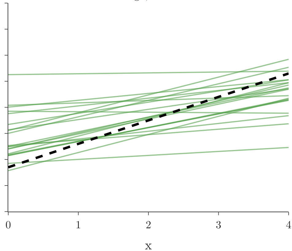
Ridge, \lambda = 1
