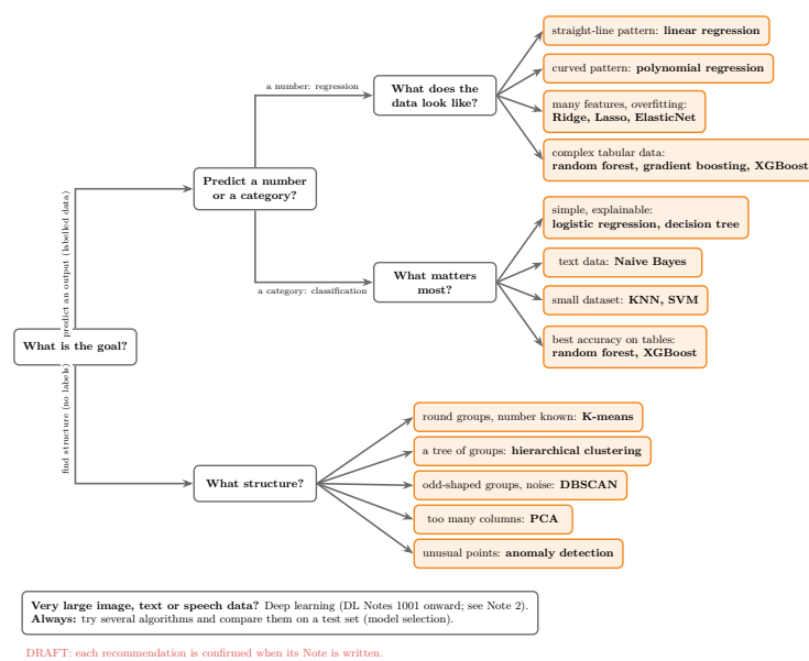
Figure 20: The Algorithm chooser (draft)
