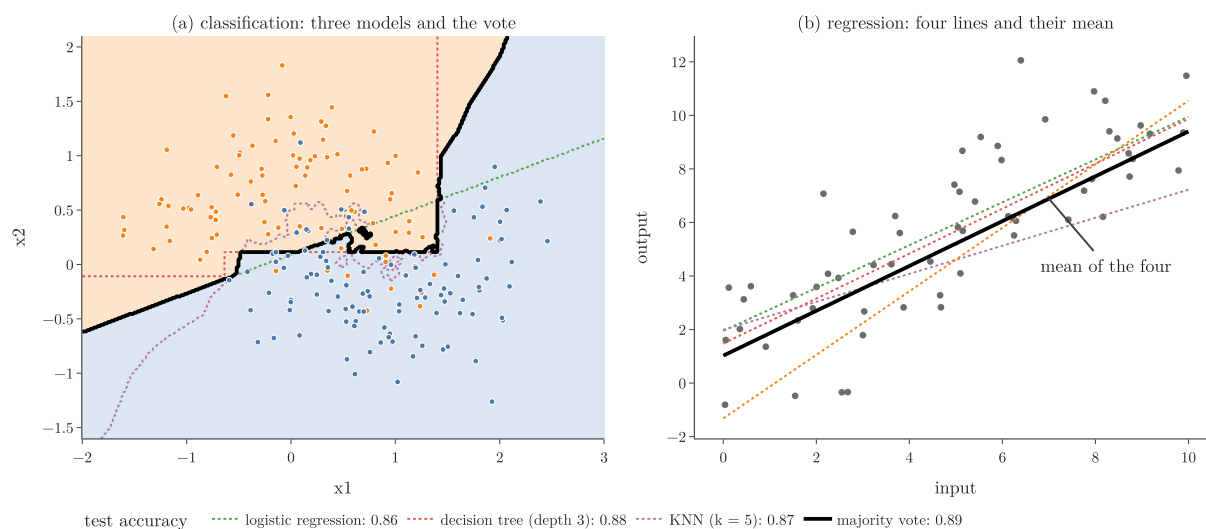
Figure 3: (a) Three classifiers' boundaries (dotted) and their majority-vote boundary (black) on two-moons data; (b) four lines, each fitted to 10 random points, and their mean
