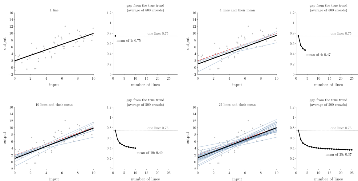
Figure 4: Lines added one at a time, each fitted to 10 random points of the same data. Left: the lines (blue), their mean (black) and the true trend (red dashed). Right: the gap between the mean line and the true trend, averaged over 500 crowds
