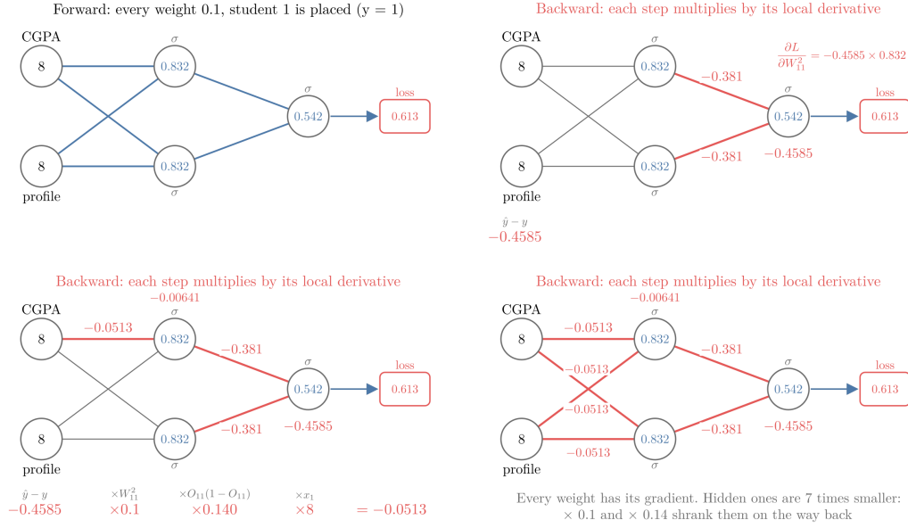
Figure 3: Backpropagation on the classification network for student 1. Forward, values flow left to right (blue). Backward, the gradient flows right to left (red): it starts as \hat{y} - y = -0.4585 at the output and is multiplied by one local derivative per step, \times 0.1 along W_{11}^2 , \times 0.140 through the hidden sigmoid, \times 8 along W_{11}^1 , until every weight holds its gradient
