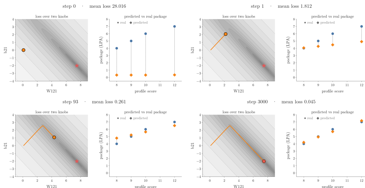
Figure 2: Gradient descent on two of the nine knobs at once, W_{21}^1 and b_{21} , over all four students; the other seven stay at their starting values. Left: the path on the contours of the mean loss (the star is the lowest point). Right: the predicted packages (diamonds) move onto the real ones (dots). Learning rate 0.2.
