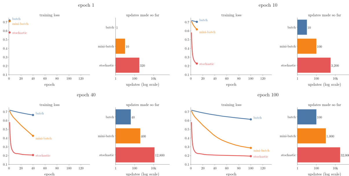
Figure 2: The three variants race for 100 epochs on the same network and data. Left: training loss after each epoch. Right: the updates each variant has made so far (log scale): 1, 10 and 320 per epoch.
