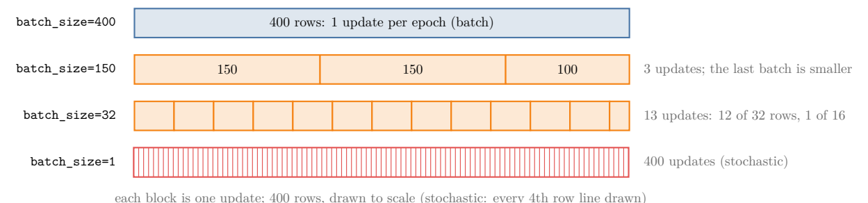
Figure 1: How Keras cuts 400 observations into batches for four values of batch_size ; each block is one update
