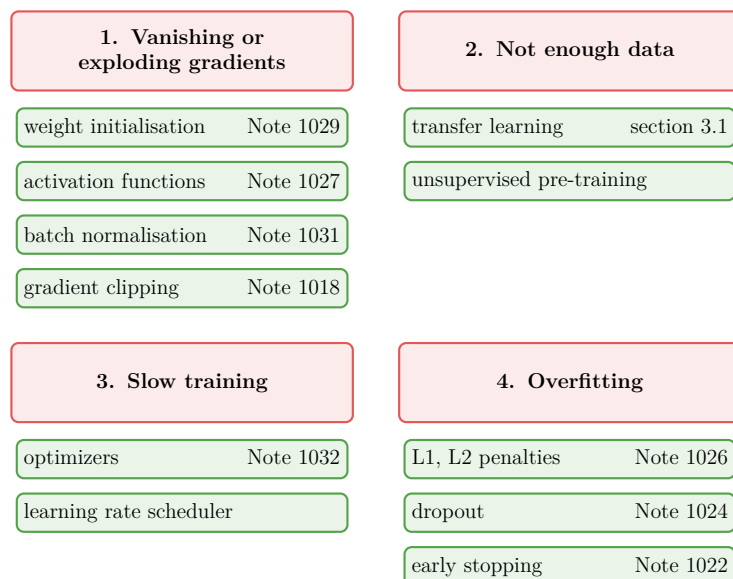
Figure 3: The four problems and where each fix is taught. Green chips name the fix and its Note
