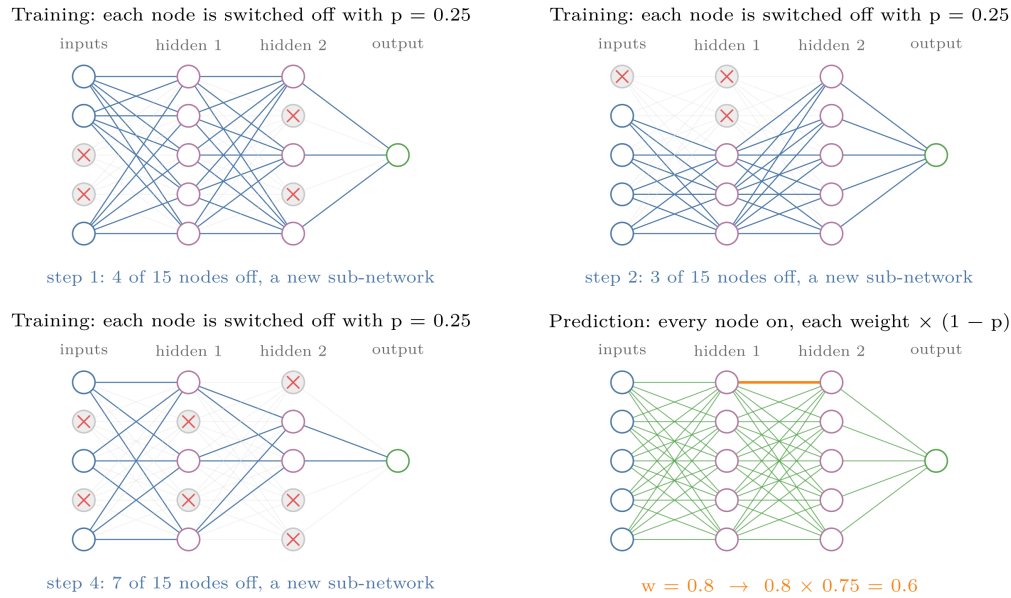
Figure 2: Dropout with p = 0.25 on the network of Figure 1, over four training steps. Each step draws a new random set of switched-off nodes (red crosses), and their connections go grey. At prediction every node is back, and each weight is multiplied by 1 - p = 0.75
