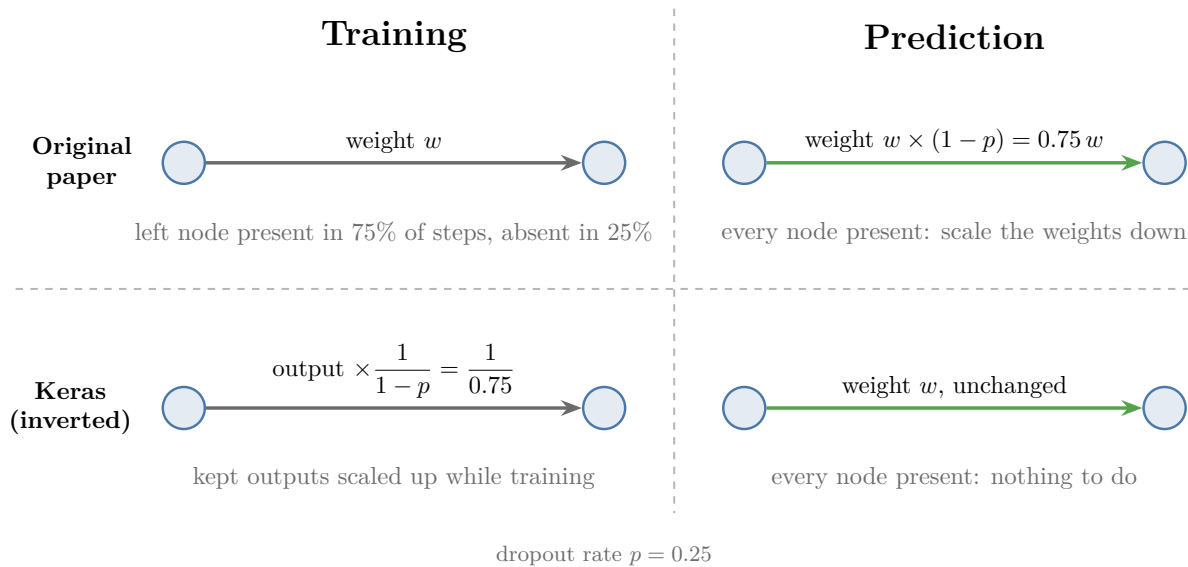
Figure 3: Two equivalent ways to handle dropout. Top: the original paper scales the weights down at prediction. Bottom: Keras scales the kept outputs up during training, so nothing changes at prediction.
