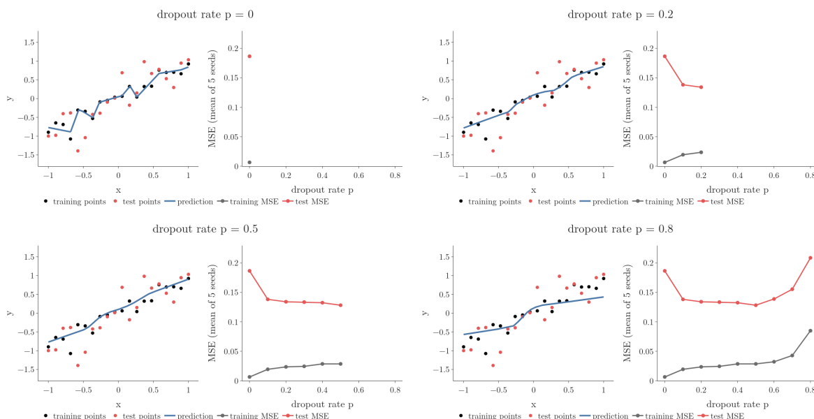
Figure 4: Dropout rate sweep on the regression problem. Left: the network’s prediction for one seed. Right: training and test MSE, mean of 5 seeds, traced as p grows from 0 to 0.8
