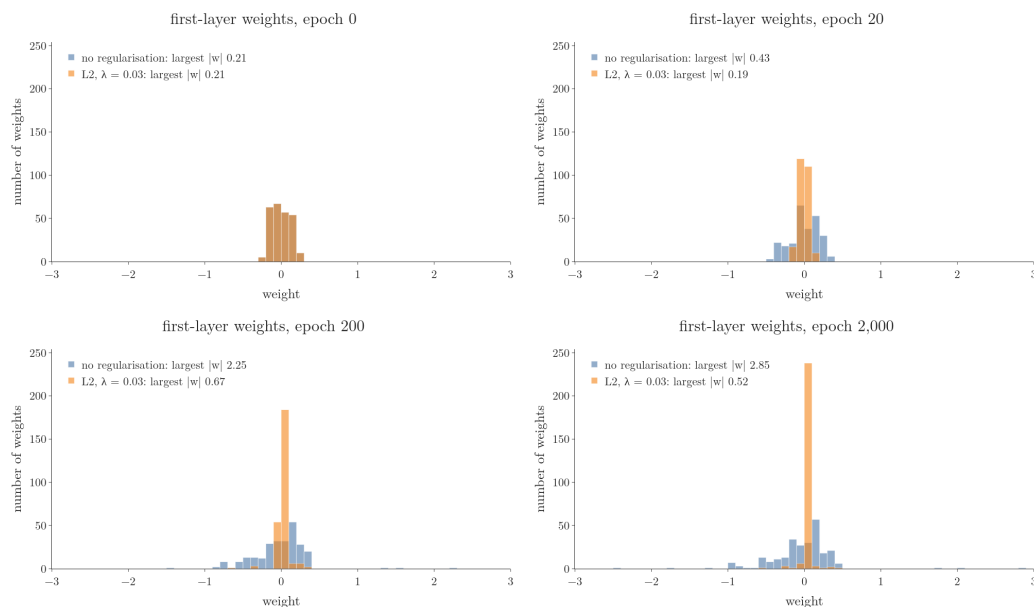
Figure 5: The 256 first-layer weights during training, same start: without regularisation (blue) they spread out, up to 2.85 in size; with L2, \lambda = 0.03 (orange), they stay in a spike around 0
