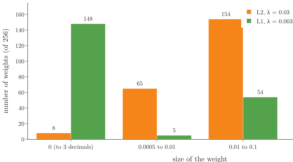
Figure 6: The 256 first-layer weights after 2,000 epochs of plain gradient descent, grouped by size: L2 (orange) and L1 (green), first random start.
