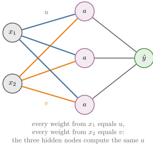
(a) Same start, three nodes
