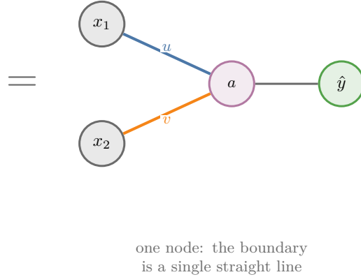
Figure 2: (a) After a start where all weights are equal, every weight leaving x_1 has one value u and every weight leaving x_2 one value v , so the hidden nodes all compute the same a . (b) The network behaves like a single hidden node
