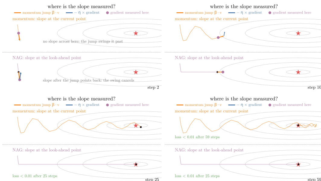
Figure 3: Momentum (top) and NAG (bottom) step by step on the valley of Figure 1. Orange: the jump \beta v_{t-1} ; blue: -\eta times the gradient; purple dot: where the gradient is measured. Momentum measures at the current point, NAG at the look-ahead point
