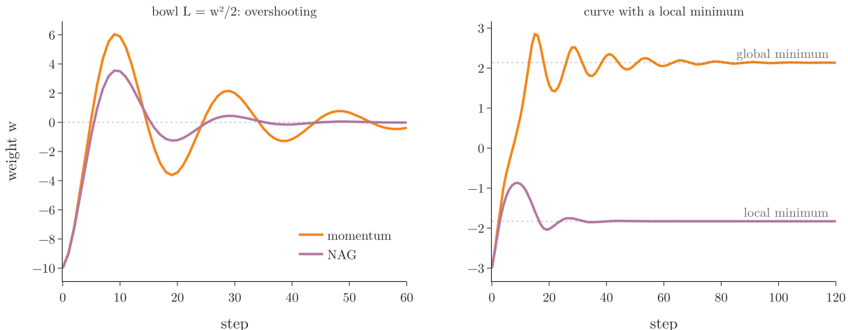
Figure 4: The weight over the steps. Left: the bowl L = w^2/2 from w = -10 , \eta = 0.1 , \beta = 0.9 ; NAG (purple) swings less far past the minimum and settles sooner than momentum (orange). Right: a curve with a local minimum from w = -3 , \eta = 0.05 , \beta = 0.9 ; momentum rolls on to the global minimum, NAG stays in the local one
