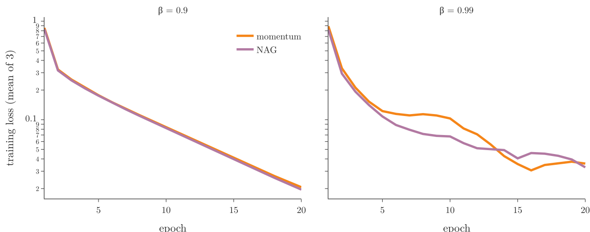
Figure 5: Training loss on MNIST per epoch, mean of 3 seeds. Left: \beta = 0.9 , the two curves overlap. Right: \beta = 0.99 , NAG (purple) mostly below momentum (orange)
