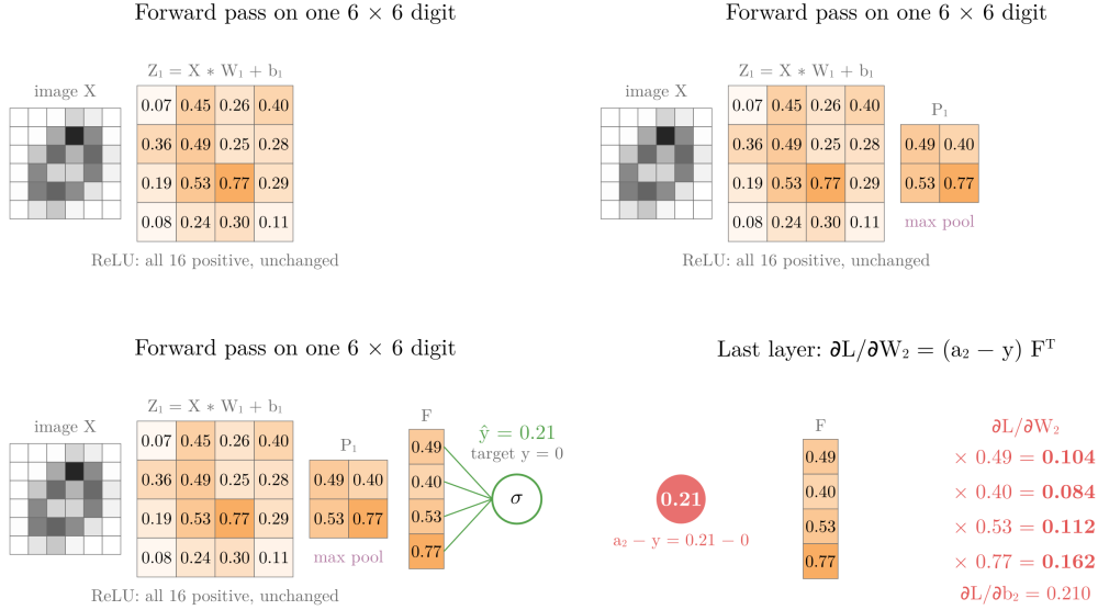
Figure 2: The Notebook's first image, a 0 shrunk to 6 \times 6 , through the small CNN with the Notebook's starting weights. The 3 \times 3 filter slides over X to fill Z_1 ; ReLU changes nothing here, since all 16 values are positive; each 2 \times 2 window sends its maximum to P_1 ; flatten gives F and the sigmoid gives \hat{y} = 0.21 . Then the error a_2 - y = 0.21 multiplies each value of F to give \partial L / \partial W_2
