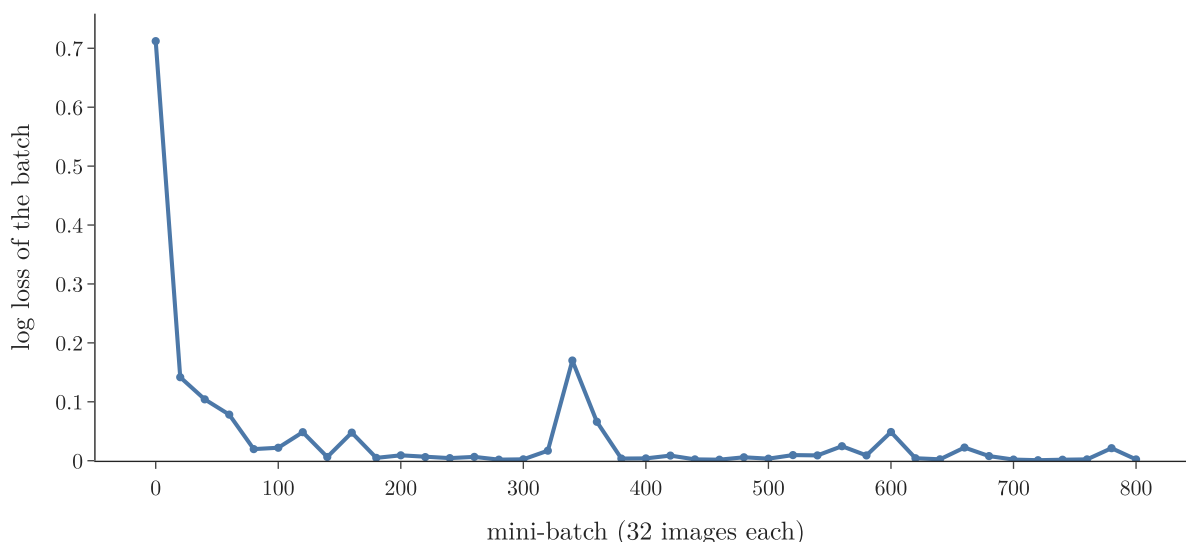
Figure 4: The loss of the batch while training with the hand-derived gradients; it drops from 0.71 to near 0 within the first few hundred mini-batches
