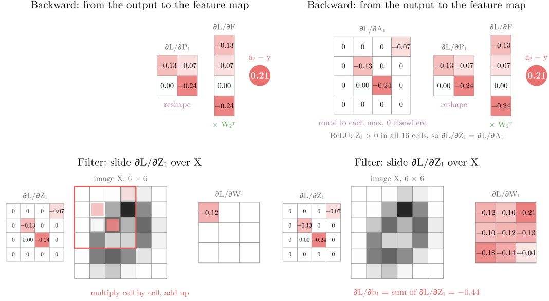
Figure 3: The whole backward pass on the 6 \times 6 digit of the part 1. Note, with the same weights. The error a_2 - y = 0.21 is multiplied by W_2^T , reshaped to 2 \times 2 , and routed to the maximum of each pooling window of A_1 . ReLU passes everything here, because all 16 values of Z_1 are positive. Then \partial L / \partial Z_1 slides over X like a filter: each position fills one cell of \partial L / \partial W_1 .
