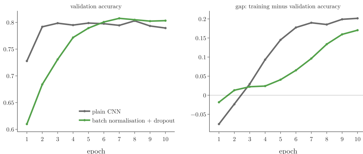
Figure 4: Plain CNN (grey) against the same CNN with batch normalisation and dropout (green): validation accuracy (left) and the gap between training and validation accuracy (right), means of 3 seeds
