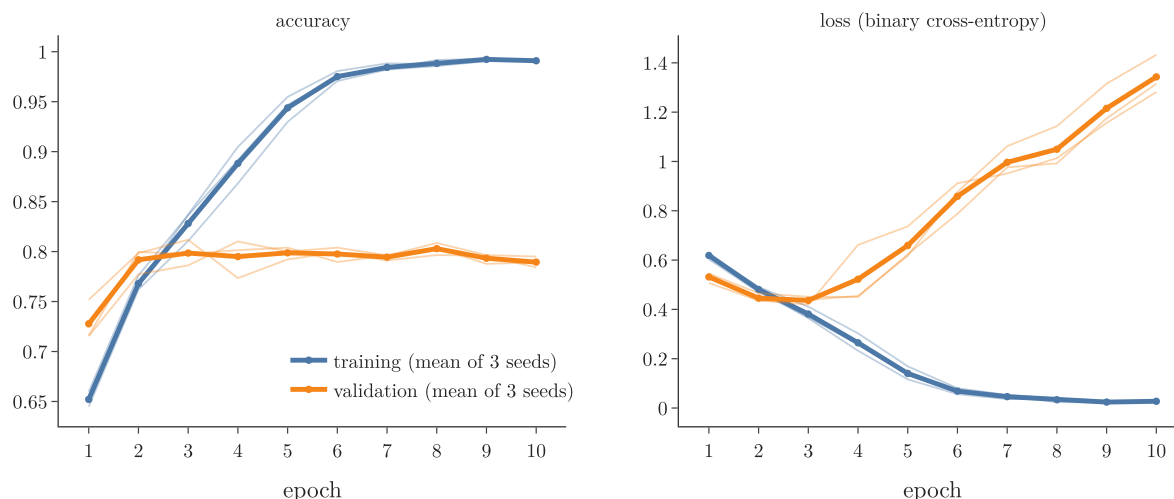
Figure 3: The plain CNN: training (blue) and validation (orange) accuracy and loss over 10 epochs. Thin lines: 3 runs with different seeds; thick lines: their mean
