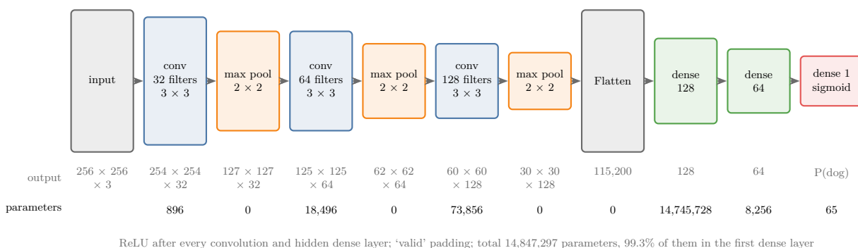
Figure 2: The CNN: three convolution (blue) and max-pooling (orange) blocks, Flatten, and three dense layers. Under each layer: its output size and its number of parameters
