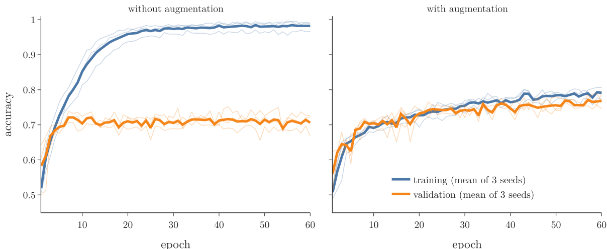
Figure 4: Training (blue) and validation (orange) accuracy without (left) and with (right) augmentation, 2,000 training photos. Thin lines: 3 seeds; thick lines: their mean
