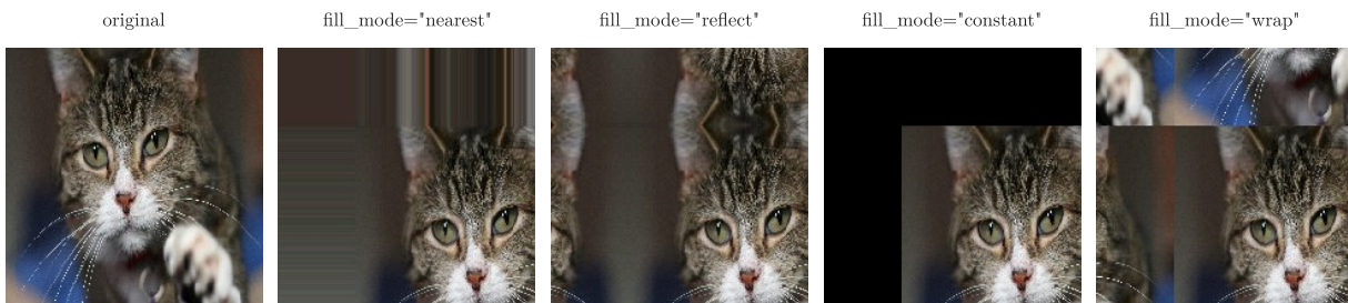
Figure 3: The photo shifted 30% right and down, with the empty pixels filled in four ways
