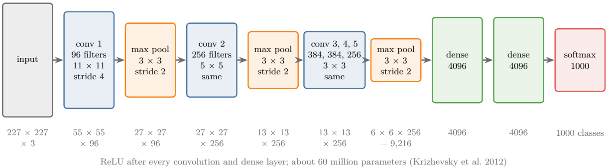
Figure 3: AlexNet: five convolution layers (blue), three max-pooling layers (orange), two dense layers of 4,096 nodes (green) and a 1,000-way softmax output (red). Under each layer: the size of its output
