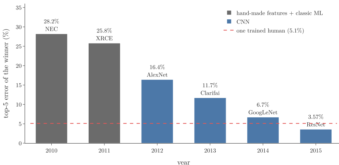
Figure 2: The winning top-5 error of ILSVRC, 2010 to 2015. Grey: classic machine learning on hand-made features. Blue: CNNs. Dashed: one trained human annotator
