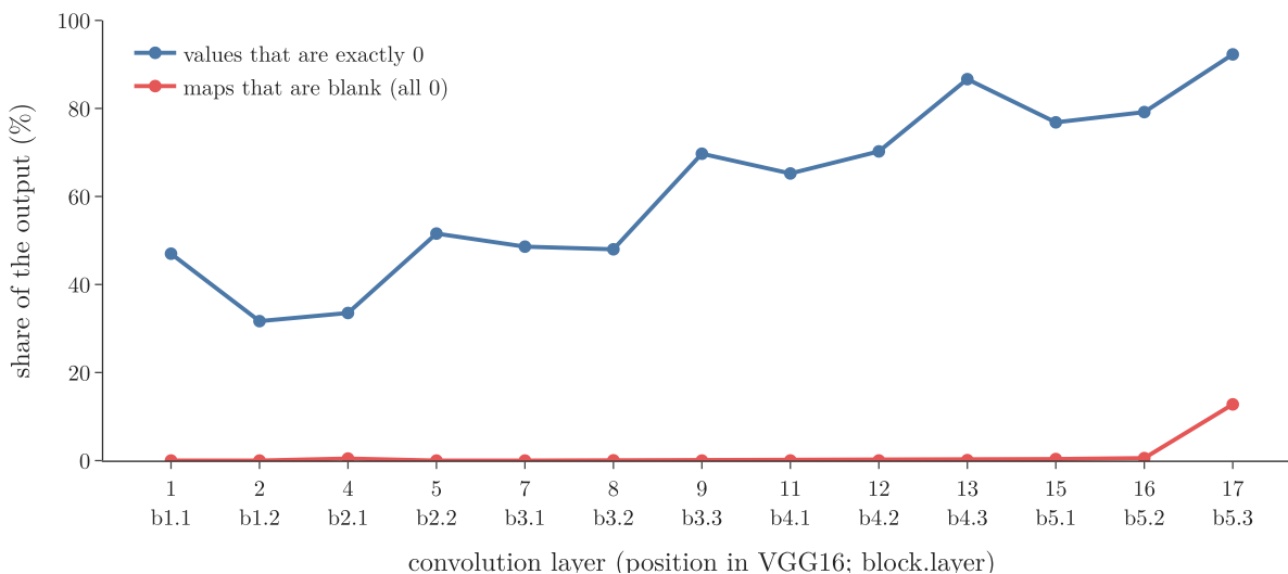
Figure 5: Share of VGG16’s convolution outputs that are exactly 0 (blue) and share of feature maps that are entirely 0 (red), averaged over 500 photos of cats and dogs
