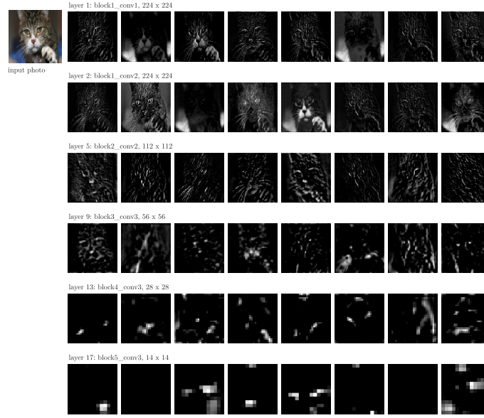
Figure 4: A kitten photo (Wikimedia Commons, David Corby, CC BY 2.5) and the first 8 feature maps it produces at six layers of VGG16. Brighter means a larger value; black means 0
