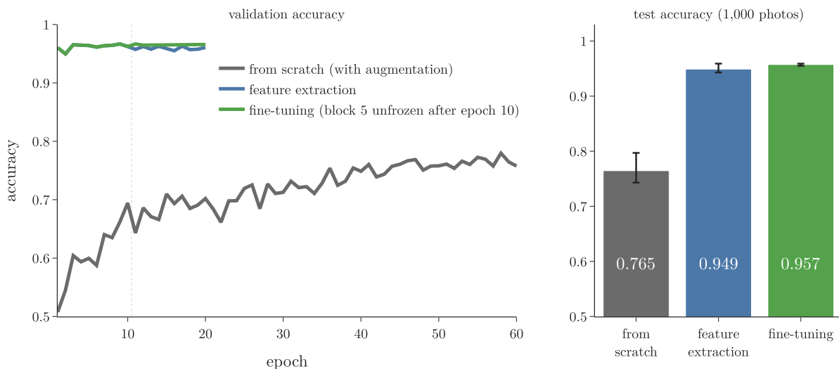
Figure 2: Validation accuracy per epoch (left; mean of 3 seeds) and test accuracy (right; bars: mean, whiskers: lowest and highest of 3 seeds). The dotted line marks where fine-tuning unfreezes block 5
