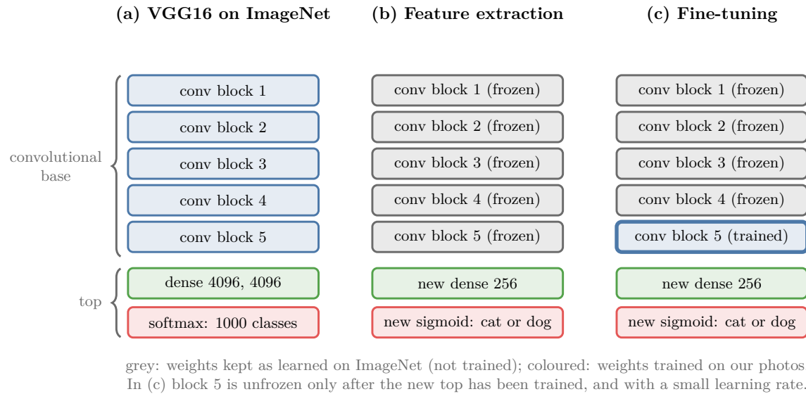
Figure 1: (a) VGG16 as trained on ImageNet. (b) Feature extraction: the whole convolutional base is frozen, and only a new top is trained. (c) Fine-tuning: the last convolution block is also trained, after the new top
