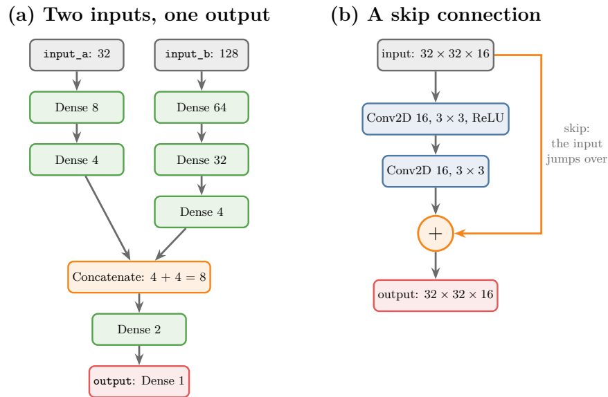
Figure 3: (a) Two inputs processed separately and joined by Concatenate . (b) A skip connection: the input jumps over two convolution layers and is added to their output
