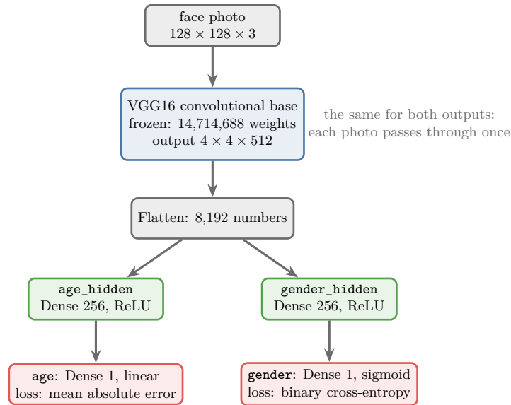
Figure 4: The age and gender model: one frozen VGG16 base, Flatten, and two branches with their own output and loss
