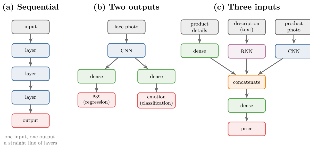
Figure 1: (a) A Sequential model is one straight line. (b) One input, two outputs: a face photo gives both an age and an emotion. (c) Three inputs, one output: product details, a text description and a photo together give a price
