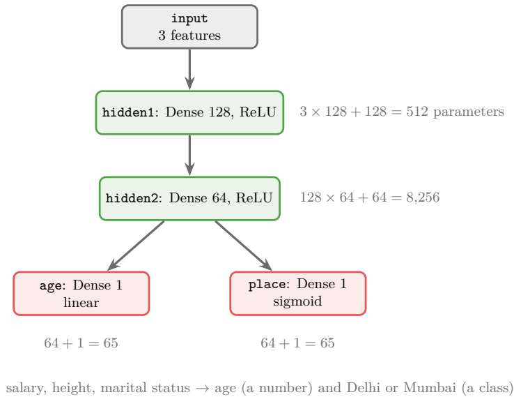
Figure 2: A functional model with one input and two outputs. Both outputs read the second hidden layer. The numbers are each layer's parameters
