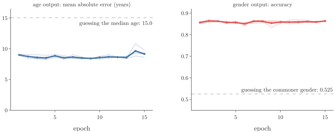
Figure 5: The two-output model on the test photos, epoch by epoch: the age error (left) and the gender accuracy (right). Thin lines: 3 seeds; thick lines: their mean; dashed: guessing
