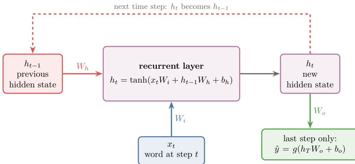
Figure 4: The simplified view of a recurrent layer. The word x_t enters through W_i , the previous hidden state through W_h ; their sum, plus the bias, goes through \tanh to give h_t , which is fed back at the next time step. After the last step, h_T goes through W_o and g to give \hat{y}
