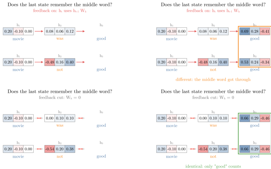
Figure 3: The test of the table, step by step. Top row “movie was good”, bottom row “movie not good”, hidden states of 3 numbers (blue for positive, red for negative). With the feedback W_h (red arrows) the two h_3 differ; with W_h = 0 (crossed arrows) they are identical
