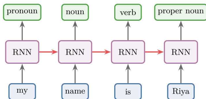
Figure 3: Many-to-many with the same length, unrolled: each time step takes one word and gives one tag
