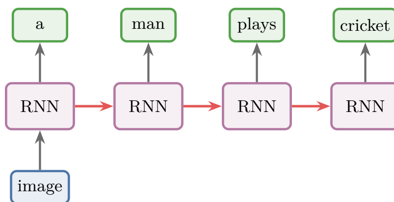
Figure 2: One-to-many, unrolled: the image enters at the first time step only; every time step produces one word of the caption
