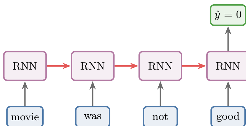
Figure 1: Many-to-one, unrolled: one word enters at each time step, the hidden state passes to the next step (red arrows), and only the last step produces an output
