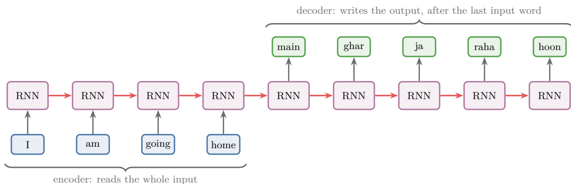
Figure 4: Many-to-many with different lengths, unrolled: the encoder reads all 4 English words; only after the last one does the decoder produce the 5 Hindi words
