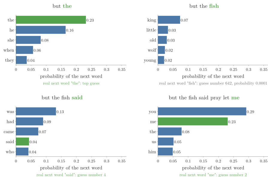
Figure 5: The sentence “But the fish said, ‘Pray let me live!’”, the first test sentence of 8 to 14 known words, typed into the model (seed 0) one word at a time. After each prefix: the model’s five most likely next words. Then the real next word appears, green when it is among the five
