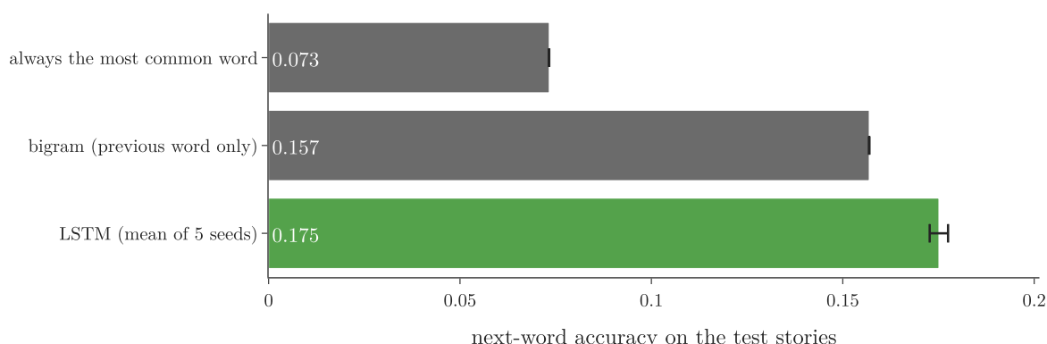
Figure 4: Next-word accuracy on the 11,366 test pairs. The LSTM bar is the mean of 5 seeds; the error bar is one standard deviation
