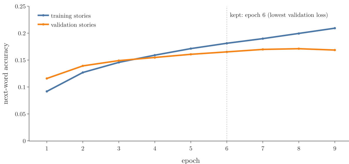
Figure 3: Next-word accuracy during training (seed 0). The dotted line marks epoch 6, the epoch with the lowest validation loss, whose weights are kept
