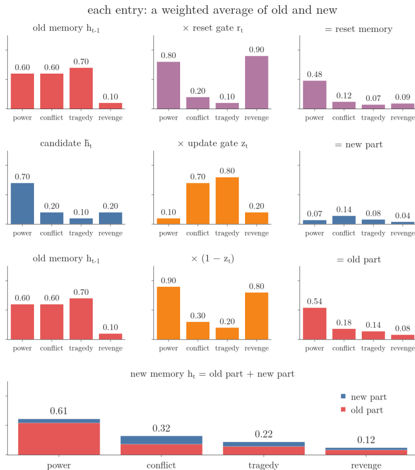
Figure 2: The four steps for sentence 4 of the story, one vector per frame. Row 1: the reset gate scales the old memory. Row 2: the update gate scales the candidate. Row 3: 1 - z_t scales the old memory. Bottom: the new memory, old part (red) plus new part (blue)
