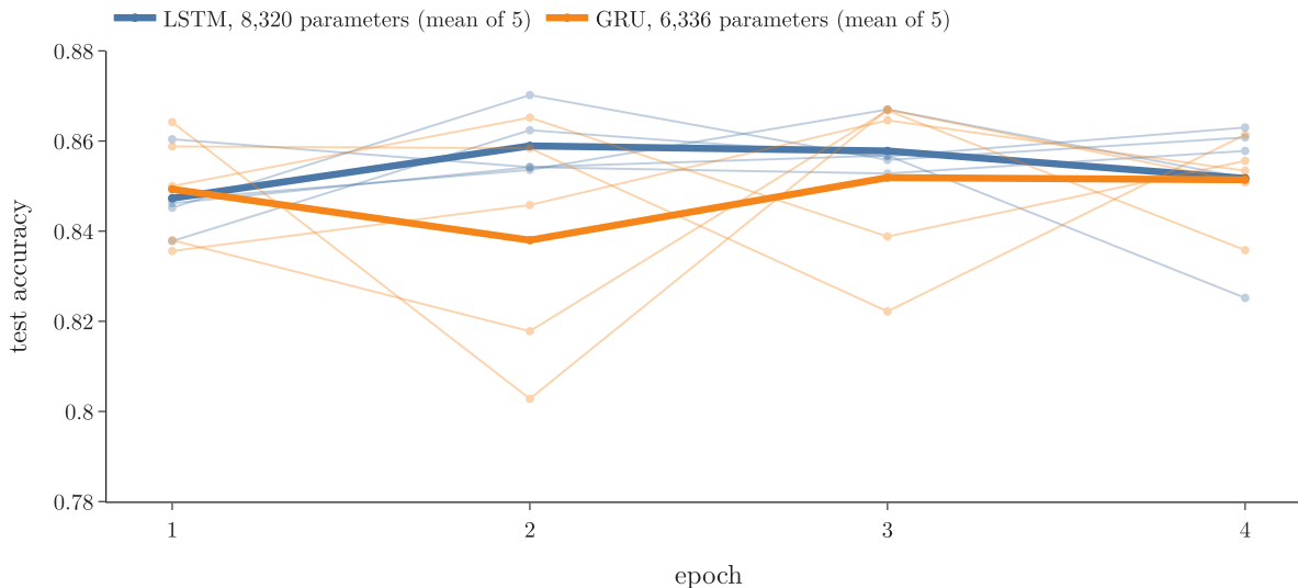
Figure 3: Test accuracy on IMDB reviews after each epoch, LSTM (blue) and GRU (orange). Thin lines: 5 runs each; thick lines: their mean. The single runs of the two models overlap; the means differ most at epoch 2 (0.838 against 0.859) and meet at epoch 4
