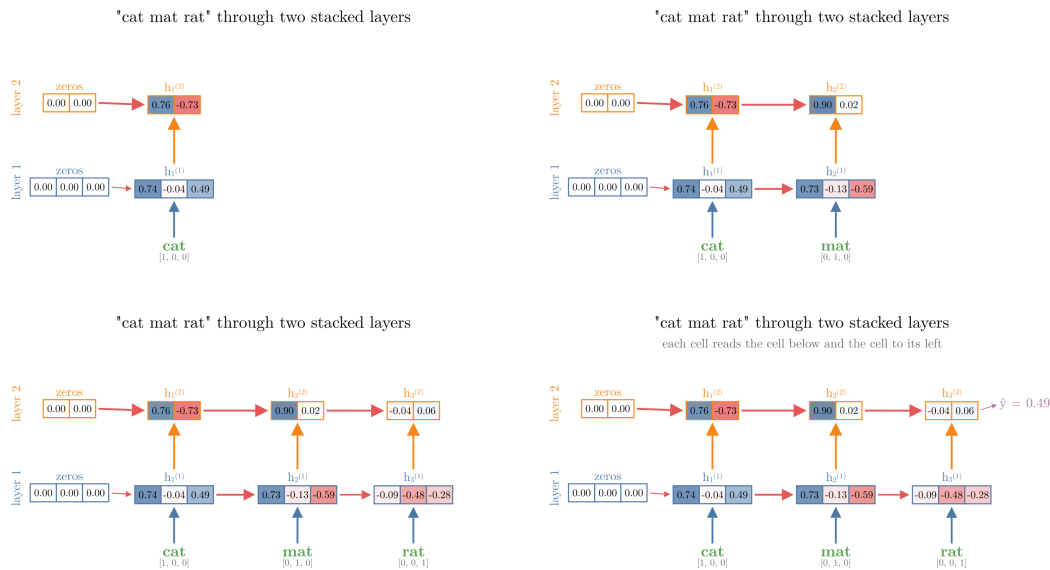
Figure 2: The two-layer stack of this section reading “cat mat rat”. At each time step the word enters layer 1 (blue), whose new hidden state goes up to layer 2 (orange); each layer also takes its own previous state from the left (red arrows). Cells are blue for positive numbers and red for negative ones. The values are the Notebook’s hand forward pass with the untrained Keras weights, so the prediction \hat{y} = 0.49 is not yet meaningful
