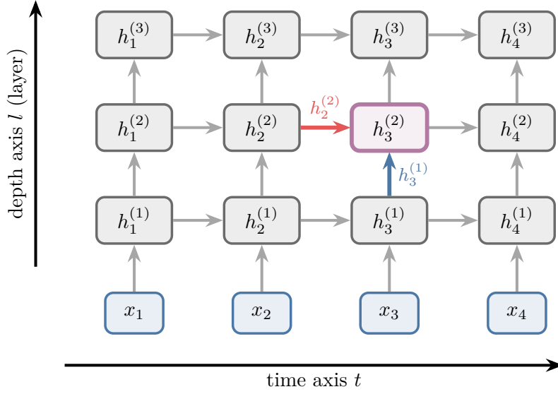
Figure 3: An unfolded deep RNN with 3 layers and 4 time steps is a grid with two axes. The highlighted cell h_3^{(2)} receives h_3^{(1)} from the layer below and h_2^{(2)} from the previous time step
