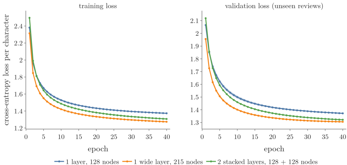
Figure 4: Training loss (left) and validation loss (right) per epoch, mean of 2 seeds (band: lower to higher seed). The loss is the cross-entropy per character, lower is better
